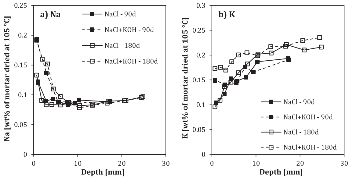
Fig. 9. Elemental profiles of a) sodium (Na), b) potassium (K), for the mortar specimens exposed to the NaCl solution (solid lines) and the NaCl+KOH solution (dashed lines) for 90 days (filled squares) or 180 days (hollow squares) given as element content [wt% of mortar dried at 105 °C] as a function of depth below the exposed surface determined with ICP-MS.
