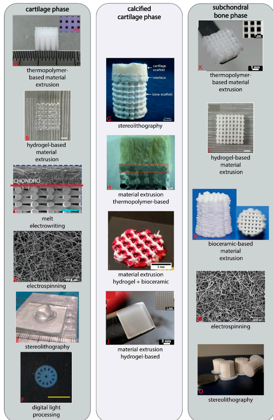
Figure 4. OC scaffold phases made via various 3D printing techniques. Some techniques, such as ME printing for thermopolymers and hydrogels, are commonly used across all phases of the OC scaffold, while other techniques, such as MEW, are commonly used only in one or two phases (cartilage and calcified cartilage). (A) Insert scale bar = 1 mm [183]. (B) Scale bar = 2 mm [113]. (C) Scale bar = 1 mm [184]. (D) Scale bar = 0.01 mm [165]. (E) [123]. (F) Scale bar = 5 mm [103]. (G) Scale bar = 2 mm [181]. (H) Scale bar = 0.5 mm [143]. (I) Scale bar = 5 mm [109]. (J) Scale bar = 2 mm, insert scale bar = 1 mm [104]. (K) Scale bar = 2 mm, insert scale bar = 1 mm [104]. (L) Scale bar = 2 mm [113]. (M) [156]. (N) Scale bar = 0.01 mm [165]. (O) [123].
