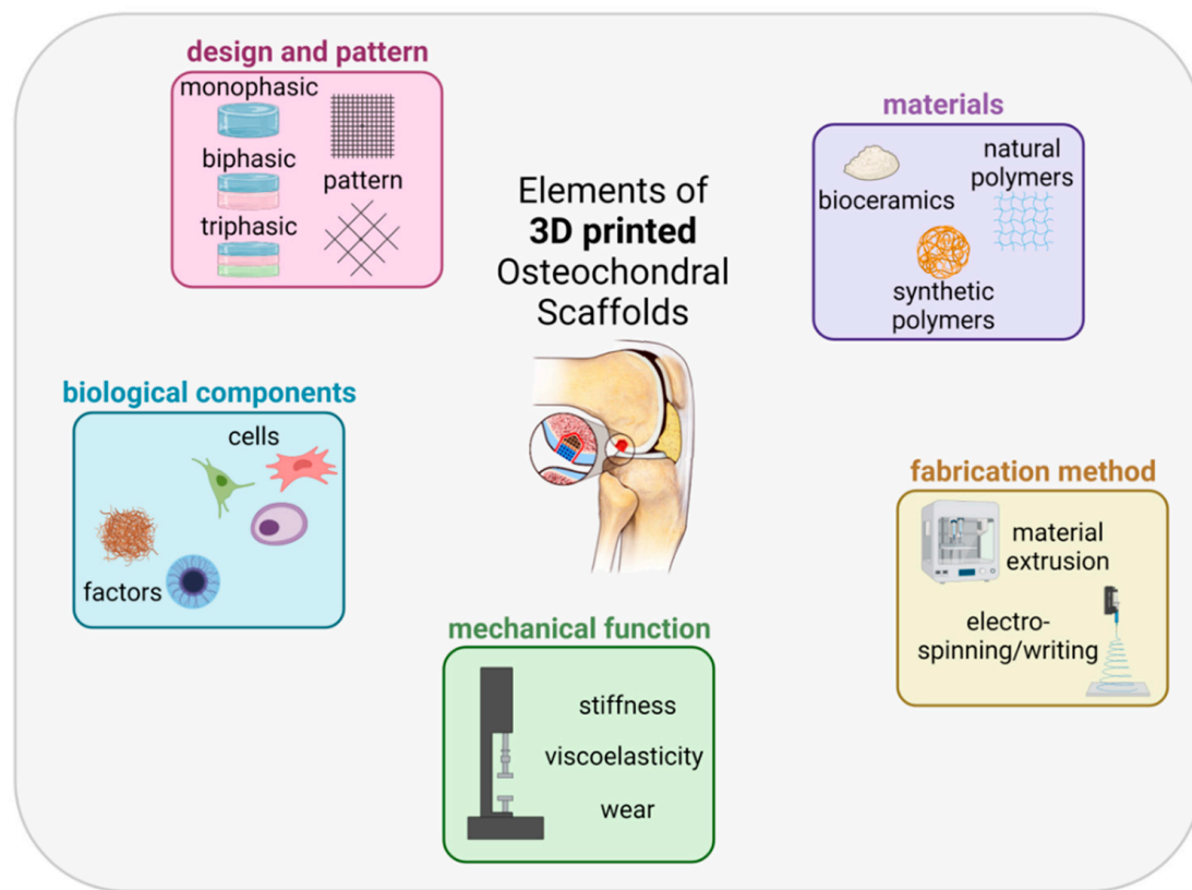
Figure 3. Elements of 3D printed OC scaffolds. We have identified five main domains of a 3D printed OC scaffold: materials (e.g., natural and synthetic polymers, bioceramics and hydrogels), fabrication method (e.g., material extrusion (ME), electro-spinning (ES), electrowriting and stereolithography (SLA)), mechanical function, biological components (e.g., cells—chondrocytes, osteoblasts, stem cells and growth factors) the overall design (e.g., mono or multiphasic) and pattern of each 3D printed layer. Figure created with BioRender.com (10 October 2021).
