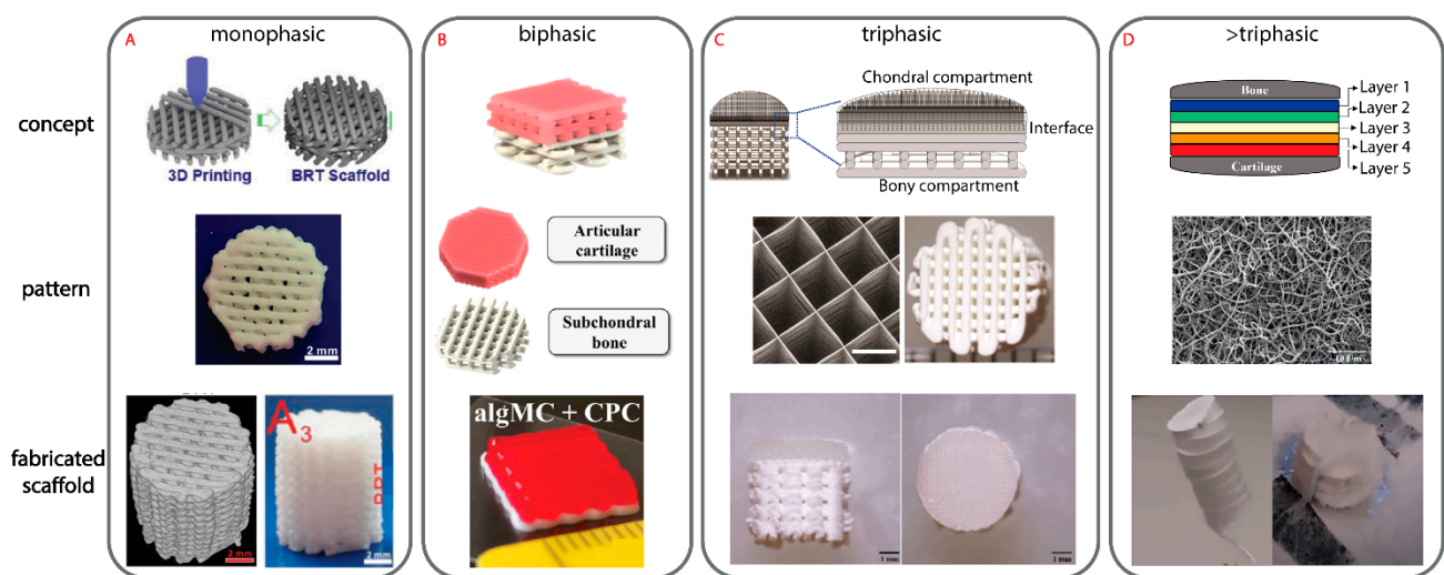
Figure 7. Examples of different scaffold design approaches including the pattern of each 3D printed layer. (A) A monophasic scaffold made from a homogenous ceramic paste ME printed. The text in the fabricated scaffold image is from the original research output [196]. (B) A biphasic scaffold with both phases ME printed. The subchondral bone phase is made from a ceramic paste and the cartilage phase is made from a hydrogel [109]. (C) A triphasic scaffold made from ME and MEW where the subchondral bone phase is made from a ceramic paste, the cartilage phase contains a thermopolymer MEW mesh and hydrogel while the interface contains all the forementioned materials [105]. (D) A >triphasic scaffold has more than three distinct phases with this example scaffold containing five individual phases all made from ES [165].
