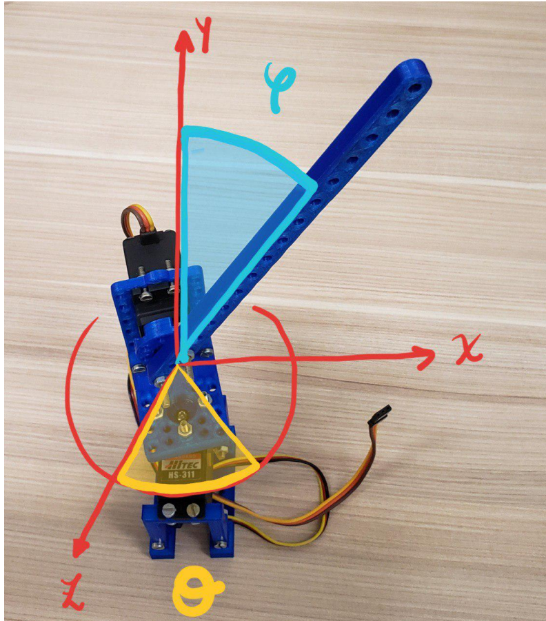
Figure 3.5 – Angles needed to control the servo motors and move the inverted pendulum
