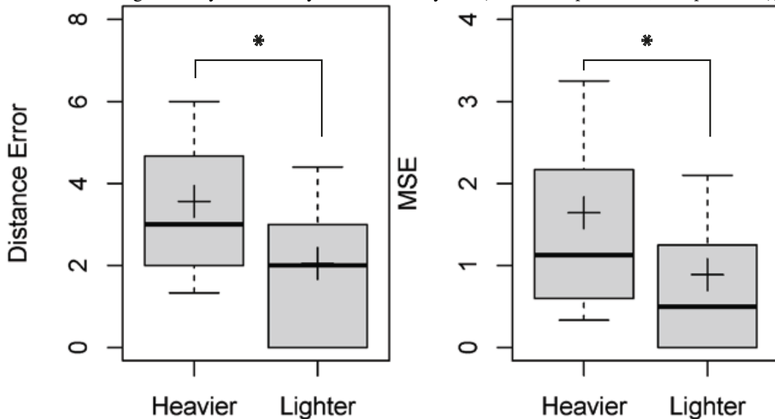
Figure 5.6 – Distance Error and the Mean Square Error for each weight group. Pairs grouped by asterisks were significantly different by Mann-Whitney test (* : 0.01 < p < 0.05 , ** : p < 0.01 )
