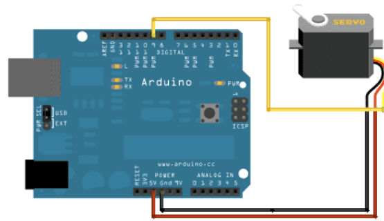
Figure 3.2 – Motor circuit
