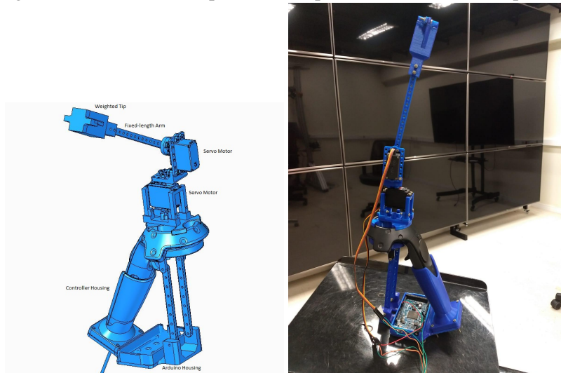
Figure 3.1 – The inverted pendulum haptic device and finished product.
