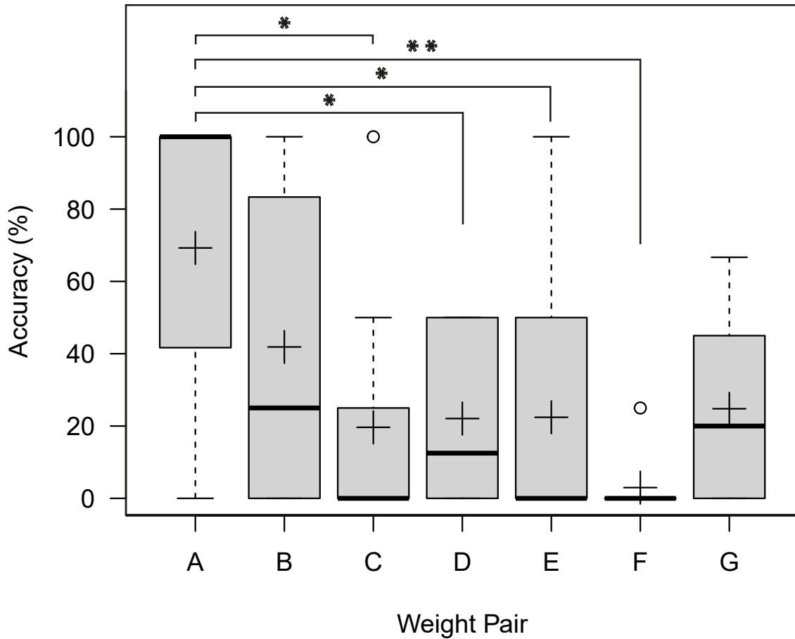
Figure 5.3 – Average percentage of correct weight pairs. Pairs grouped by asterisks were significantly different by Mann-Whitney test (* : 0.01 < p < 0.05 , ** : p < 0.01 )
