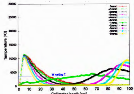
Figure 4: Temperature peaks on the tungsten insert surface for a bunch at 3.5TeV. The scan is performed using steps of 1mrad in the whole angle range.
