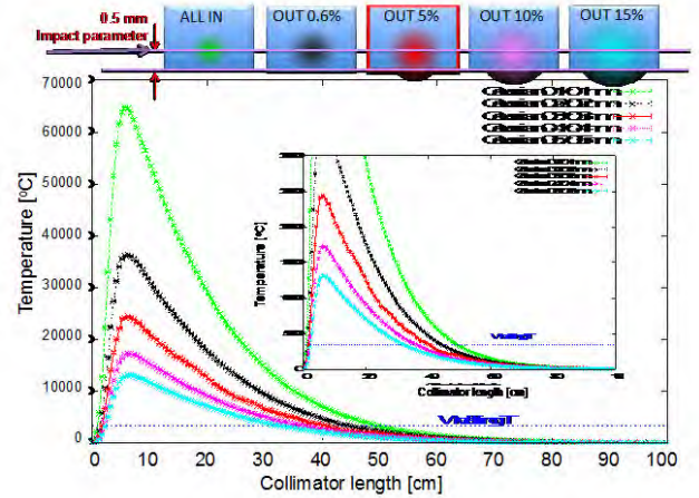
Figure 7: Temperature peaks in case of jaw-beam parallel orientation, scanning over 5 different beam sizes. In the zoomed area the temperature scale is the same as for the previous temperature graphs. Above the plot, 2D maps of the escaping protons that don't interact with the jaw due to the impact parameter chosen are shown.
