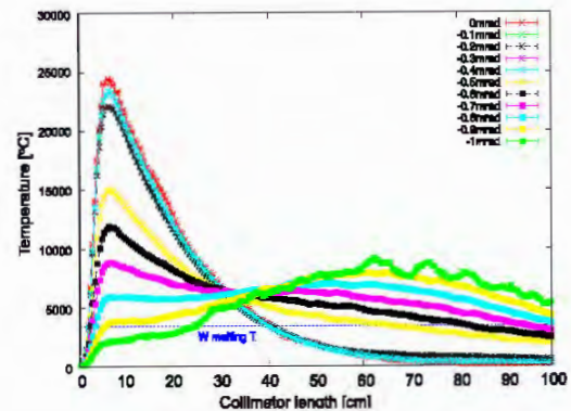
Figure 5: Temperature peaks on the tungsten insert surface for a bunch at 7TeV. The scan is performed using steps of 0.1mrad in the angle range of [0:-1] mrad.
