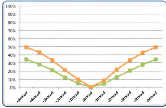
Figure 6: Fraction of escaping energetic protons (with respect to the impacting ones) for different jaw tilt angles. Orange line refers to escaping protons of energy between 1 and 7 TeV, while the green line refers to protons that have lost only 1% of the starting 7 TeV energy, after impacting the jaw.
