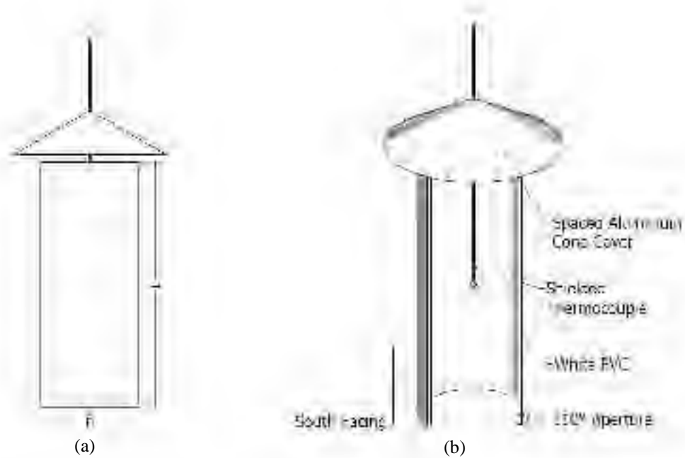
Figure 3: PVC Radiation Shields (a) Front View of Full Pipe PVC Radiation Shield (b) 3D View of PVC shield with slit aperture
