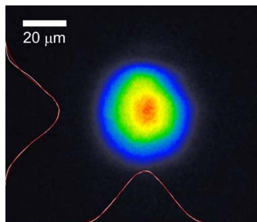
Fig. 2 Beam profile of the XeCl excimer laser.
