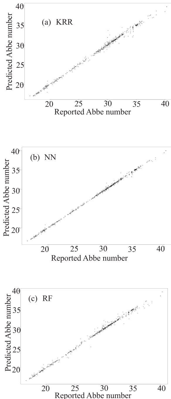
FIG. 1. Predicted Abbe number plotted against the reported Abbe number for (a) KRR, (b) NN, and (c) RF.
