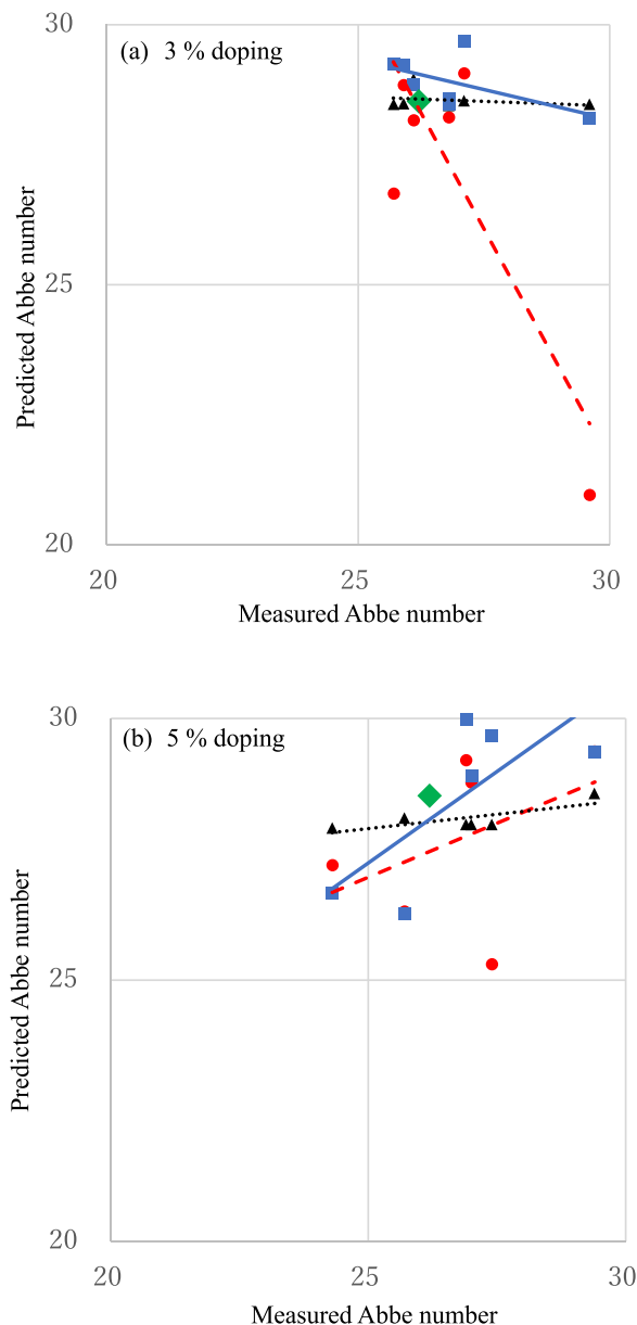
FIG. 2. Measured and predicted Abbe number for doping level of (a) 3% and (b) 5%. The blue square, red circle, black triangle, and green diamond corresponds to KRR, NN and RF, ND glass, respectively. The linear regression lines are also shown as blue straight line for KRR, red dashed line for NN and black dotted line for RF.
