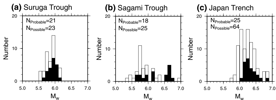
Figure 8. Moment magnitude histograms of estimated SSEs in three regions. Solid and open bars indicate the number of probable and possible SSEs, respectively. (a) Along the Suruga Trough. (b) Along the Sagami Trough. (c) Along the Japan Trench. SSE, slow slip event.
