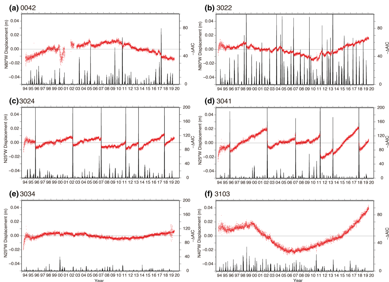
Figure 2. Cleaned coordinates at the selected GNSS stations. See Figure 1 for station locations labeled a-f. A linear trend was removed for plotting. (a) Daily coordinates (red dots) and -\Delta\text{AIC} (vertical black bars) for the \text{N}80^\circ\text{W} component at station 0042. (b) Same as (a), but for station 3022. (c) Same as (a), but for the \text{N}25^\circ\text{W} component at station 3024. (d) Same as (c), but for station 3041. (e) Same as (c), but for station 3034. (f) Same as (a), but for the \text{N}40^\circ\text{W} component at station 3103. AIC, Akaike Information Criterion; GNSS, Global Navigation Satellite System.
