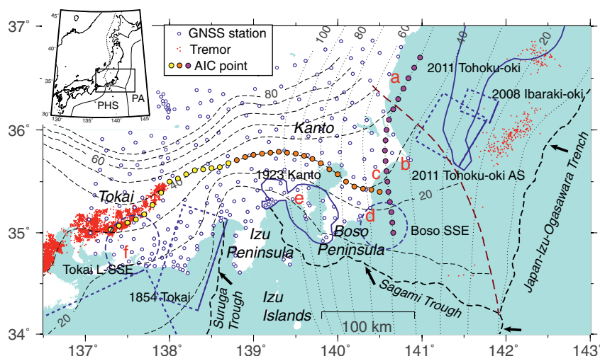
Figure 1. Map of the study area. Dashed and dotted contours are iso-depths of the plate interfaces for the Philippine Sea plate (PHS) and the Pacific plate (PA), respectively. Arrows near the trenches and troughs represent approximate directions of relative block motion (Nishimura et al., 2018). Blue circles indicate GNSS stations. The stations labeled a–f correspond to parts of Figure 2, showing the coordinate time series. Yellow, orange, and magenta circles indicate the central points of the rectangular areas used to calculate \Delta AIC averages of the N40°W, N25°W, and N80°W components, respectively. Red dots indicate tectonic tremors (Nishikawa et al., 2019; Obara et al., 2010). Source regions for the 1923 M_w 7.9 Kanto earthquake and the 2011 M_w 9.0 Tohoku-oki earthquake show 2 m (Pollitz et al., 2005) and 5 m (S. Ozawa et al., 2012) contours of coseismic slip, respectively. Rectangular fault models for the largest M_w 7.8 aftershock of the Tohoku-oki earthquake (Nishimura et al., 2011), the 2008 M_w 6.8 Ibaraki-oki earthquake (GSI, 2008), and the 1854 M_w 8.0 Ansei-Tokai earthquake (Ishibashi, 1981) are also shown. (Inset) Regional tectonic map of the study area. AIC, Akaike Information Criterion; GNSS, Global Navigation Satellite System.
