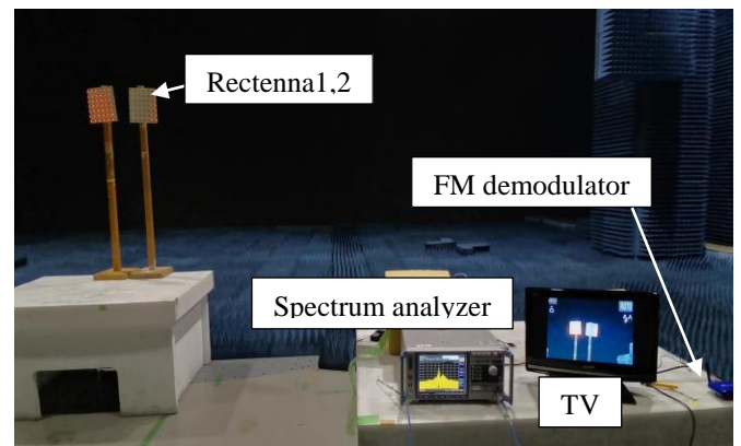
Fig. 4 Photo of the demonstration experimental setup.
