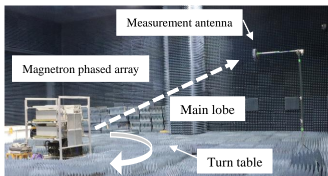
Fig. 2 Photo of the magnetron phased array system for measuring error vector magnitude.
