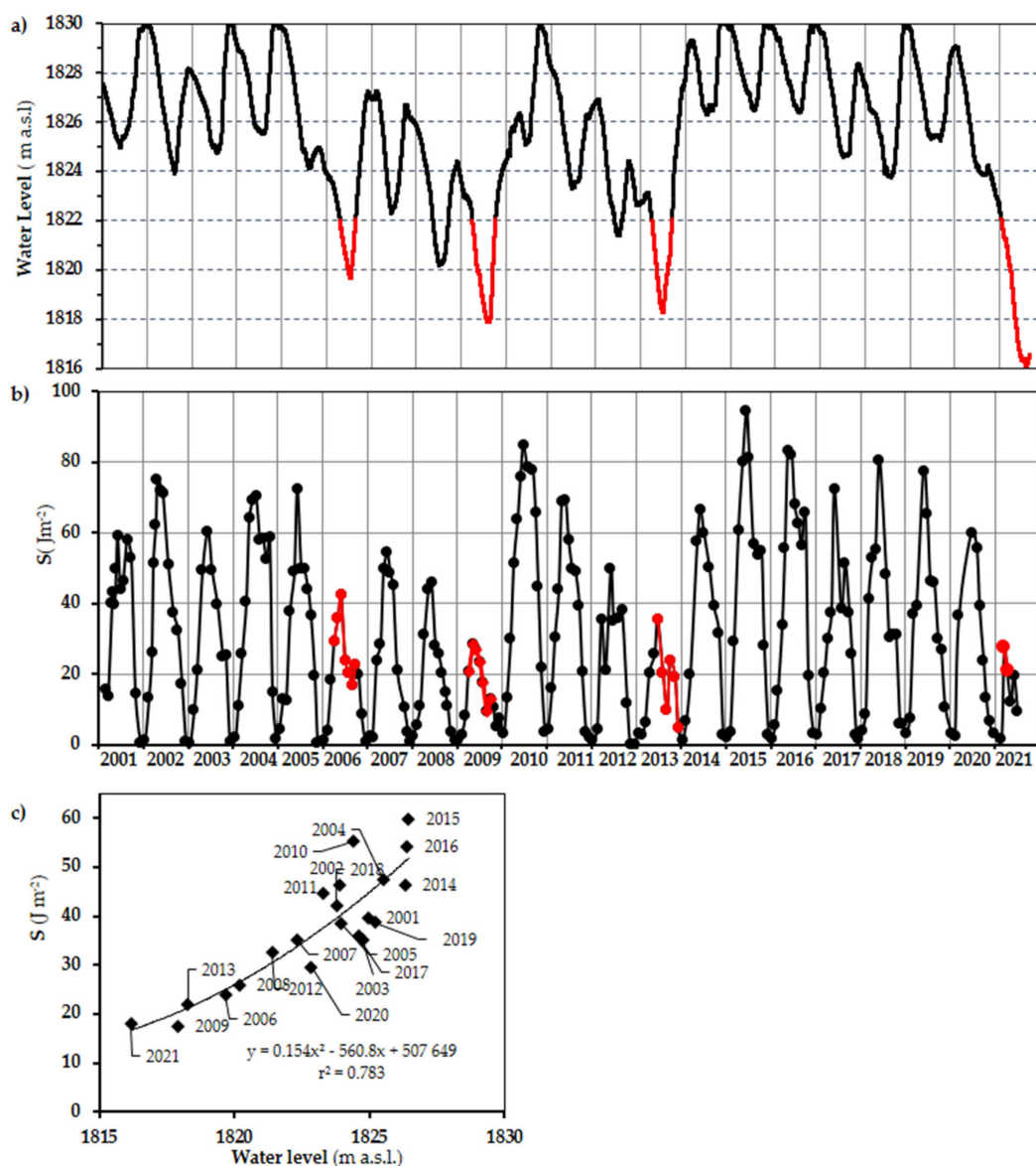
Figure 3. Time variations in VB during 2001–2021: (a) water level (daily resolution, m a.s.l.), (b) stability of stratification ( S , J m^{-2} ), and (c) relationship between mean S and minimum water level during the stratification periods. Red lines outline the four years with extraordinary minimum water levels (2006, 2009, 2013, and 2021) in some of the graphs.
