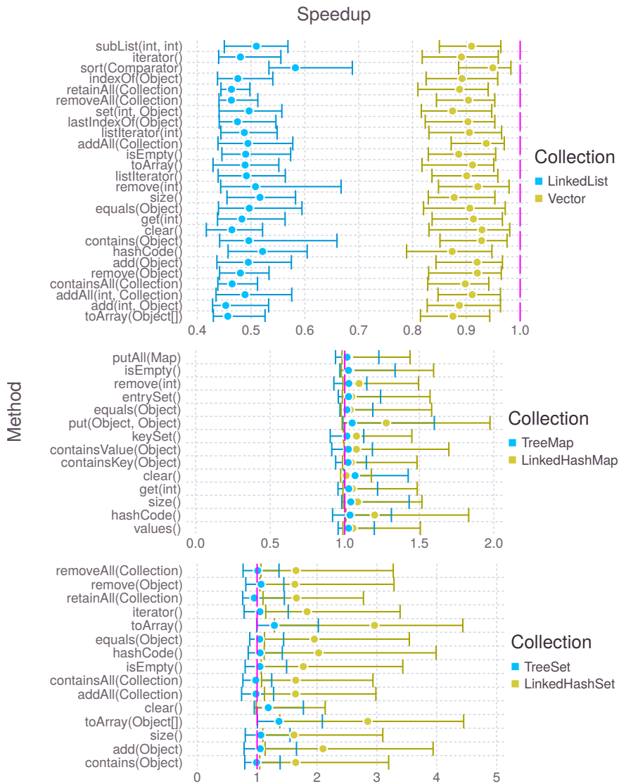
Figure 3: Median speedup of various collections compared to baseline (in magenta), with 25% and 75% quantiles
