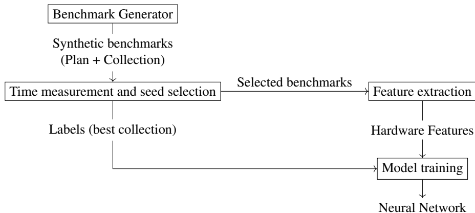
Figure 1: Overview of Brainy
