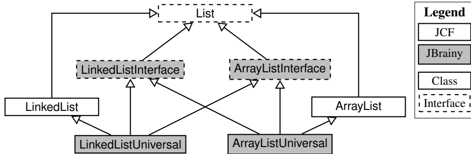
Figure 4: JBrainy subtyping hierarchy for two container classes, ArrayList and LinkedList . For each such container T , T Interface serves as general interface, and T Universal serves as implementation (extending T ) that implements all Interfaces.
