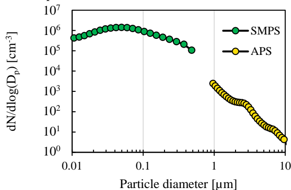
Figure 2. Number size distributions of the aerosol particles generated by the atomizer. The SMPS measured the mobility diameter (0.010-0.6 \mu\text{m} ) and the APS measured the aerodynamic diameter (0.9-10 \mu\text{m} ).
