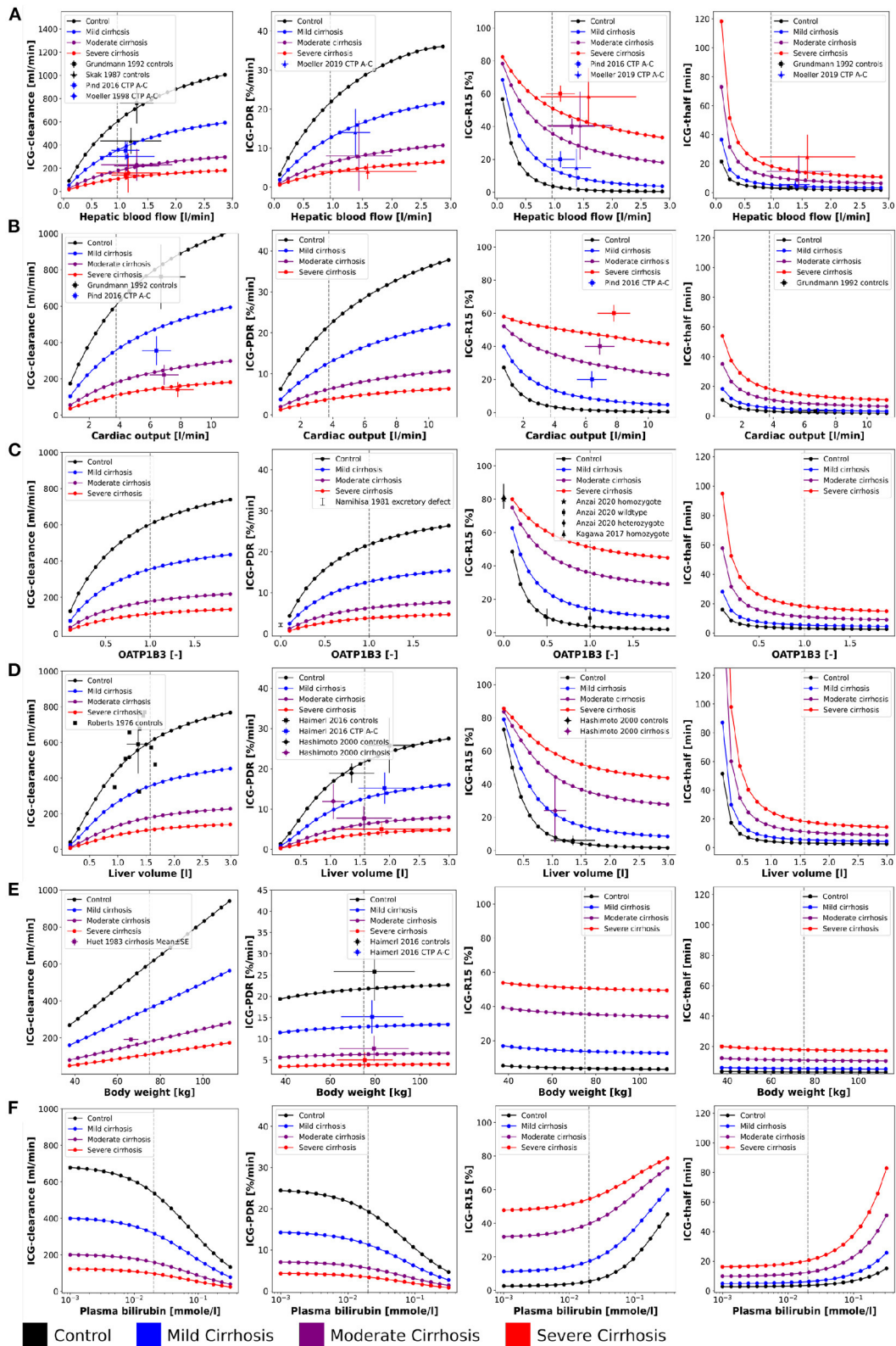
FIGURE 2 | Effect of physiological factors on ICG parameters: The effect of hepatic blood flow, cardiac output, OATP1B3, liver volume, body weight, and plasma bilirubin on ICG-clearance, ICG-PDR, ICG-R15, and ICG-t 1/2 were studied. Reference values of the model parameters, i.e., model parameters in the
