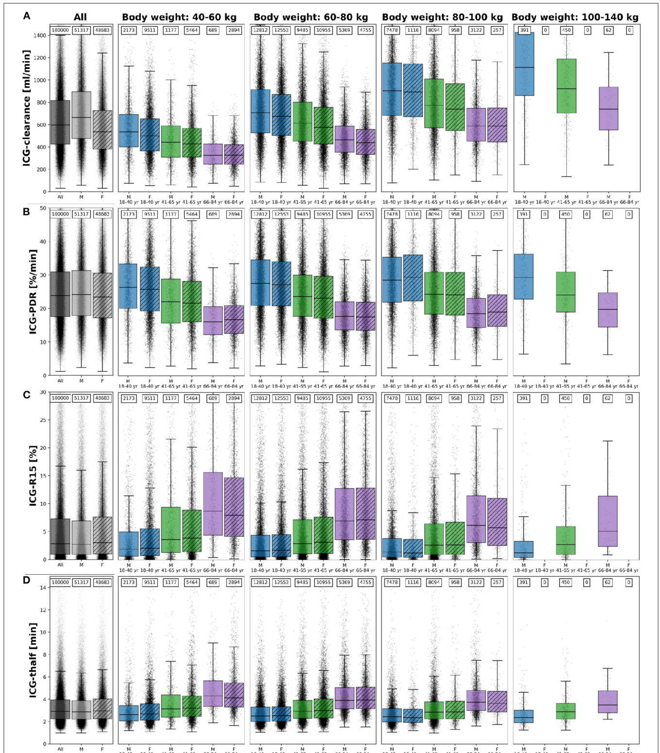
FIGURE 6 | ICG parameters healthy in silico population: The dependency of (A) ICG-clearance [ml/min], (B) ICG-PDR [%/min], (C) ICG-R15 [%], and (D) ICG-t 1/2 [min] on body weight, sex and age in n = 100,000 individuals. Results are stratified by body weight class (40–60 kg, 60–80 kg, 80–100 kg, and 100–140 kg), age group (blue, 18–40 year; green, 41–65 year; purple, 66–84 year) and sex (M, unshaded; F, shaded). No women exist with body weight > 100 kg in the cohort. The sample size of the respective subgroups are depicted above each boxplot. The box extends from the lower to upper quartile values of the data, with a line at the median with whiskers as defined by Tukey. Individual data points are plotted for all subgroups. Subjects were simulated as healthy controls. For the corresponding results in mild cirrhosis, moderate cirrhosis, and severe cirrhosis see Supplementary Figures 1–3 , respectively.
