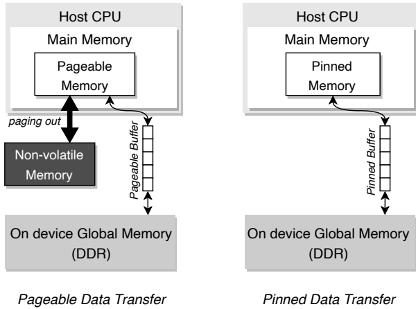
Figure 2. Pageable and Pinned Data Transfers.
