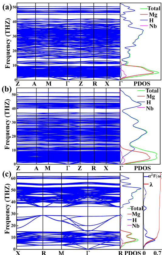
FIG. 2: (a) Phonon spectrum and projected phonon density of states (PHDOS) of (a) P\bar{4}2m - Mg_7NbH_{16} at 0 GPa, (b) P\bar{4}1 - Mg_7NbH_{19} at 0 GPa and (c) Fm\bar{3}m - Mg_7NbH_{16} at 75 GPa.
