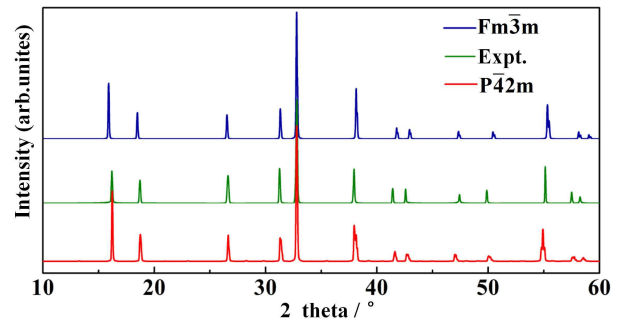
FIG. 4: Simulated XRD patterns for Mg_7NbH_{16} with space group P\bar{4}2m and Fm\bar{3}m compared with experiment from Ref. 30.
