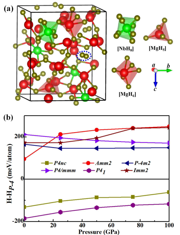
FIG. 7: (a) Crystal structure and local metal environments of Mg_7NbH_{19} at ambient pressure. (b) Relative formation enthalpies per atom in Mg_7NbH_{19} as function of pressure.
