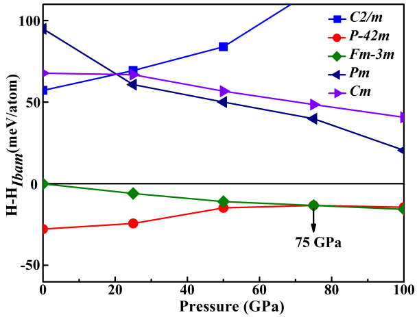
FIG. 5: Enthalpy curves per atom in \text{Mg}_7\text{NbH}_{16} as function of pressure relative to Ibam structure.
