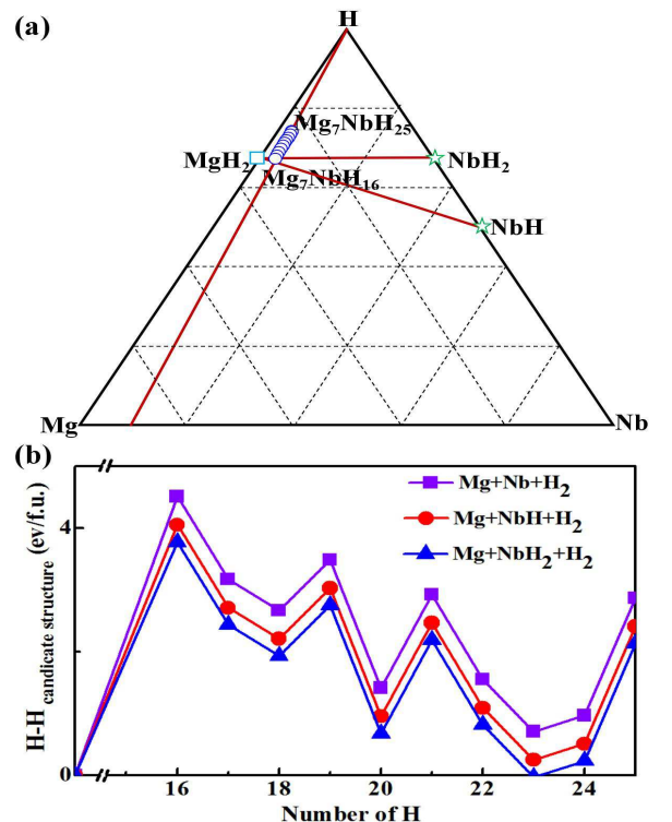
FIG. 1: (a) The ternary phase diagram for Mg-Nb-H system at ambient pressure. (b) Enthalpies per formula unit in \text{Mg}_7\text{NbH}_n ( n=16-25 ) as function of number of H with respect to the predicted candidate structures for each stoichiometry.
