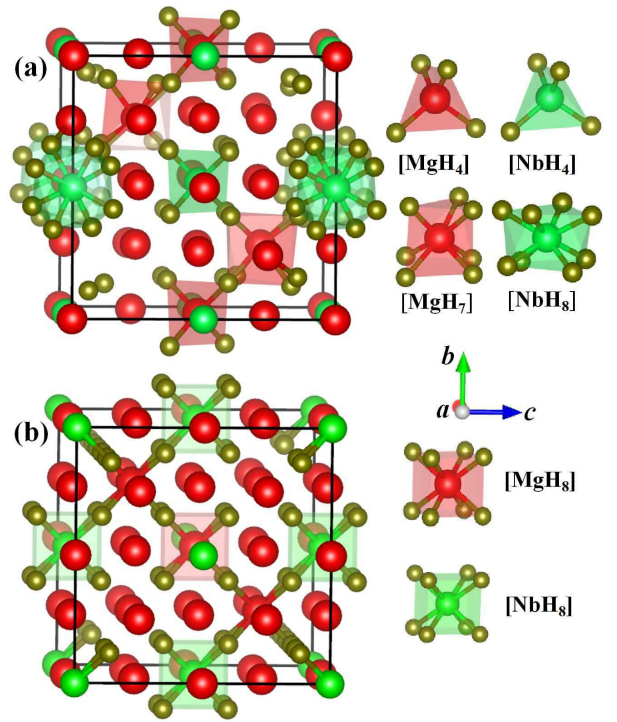
FIG. 3: Crystal structures and local metal environments of Mg_7NbH_{16} at (a) 0 GPa ( P\bar{4}2m ) and (b) 75 GPa ( Fm\bar{3}m ). Red, green and yellow spheres represent Mg, Nb and H atoms, respectively.
