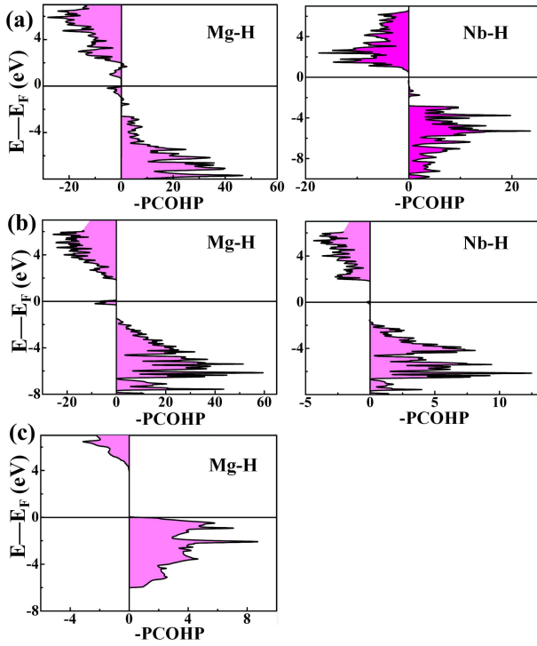
FIG. 6: Calculated -COHP curves for per Mg-H and Nb-H bond in unit cell: (a) -COHP for \text{Mg}_7\text{NbH}_{16} ; (b) -COHP for \text{Mg}_7\text{NbH}_{19} and (c) -COHP for \text{MgH}_2 .
