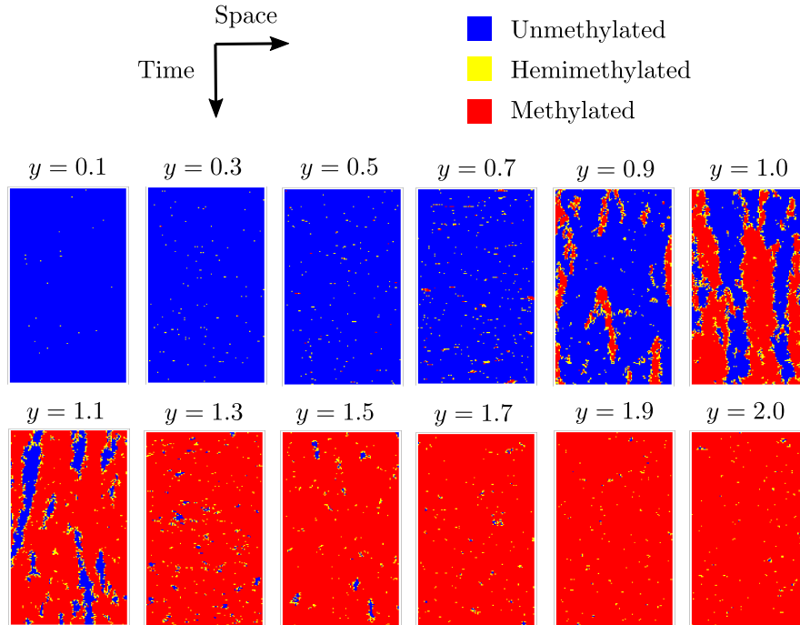
Figure 10: Size of unmethylated ( u ) clusters and methylated ( m ) clusters are most similar when y = 1 . Visualisations of stochastic simulations over time for different values of y . For each y , the horizontal axis shows simulated methylation patterns for 100 CpGs when x = 50 from the full nearest-neighbour collaborative system (see Section 2.2). The vertical axis shows patterns obtained at successive time points after steady state has been reached where timepoints are taken at constant time intervals.
