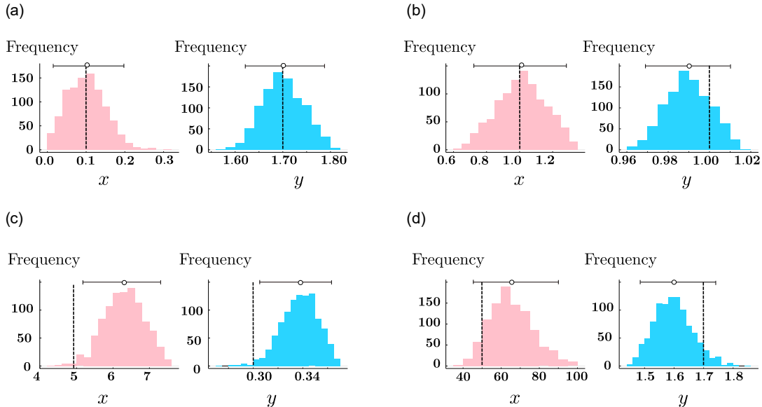
Figure 11: The OPMF model can be used to infer collaborativity and methylation strengths. Example posteriors from inference are shown, with (a), (b), (c) and (d) each corresponding to a different parameter set. True parameter values are denoted by dashed lines, inferred parameter values are shown as dots, with 95% confidence intervals shown as horizontal bars.
