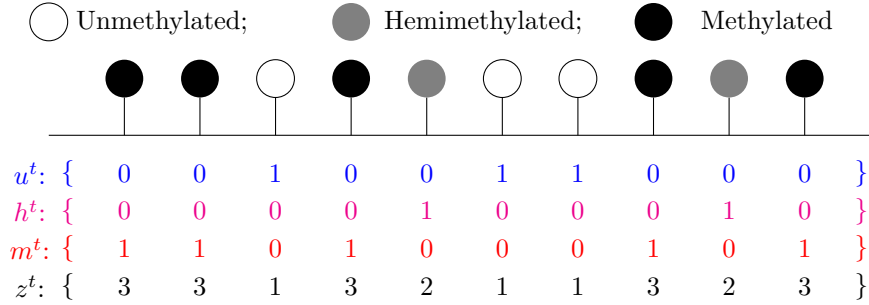
Figure 4: Construction of the sequences u^t , h^t , m^t and z^t . For simplicity, only ten CpGs are shown for a single timepoint, t . A vector u^t is created, where u_i^t = 1 if CpG i is unmethylated at time t and u_i^t = 0 otherwise. Vectors h^t and m^t are constructed similarly. Finally, a vector z^t is created via z^t = u^t + 2h^t + 3m^t .
