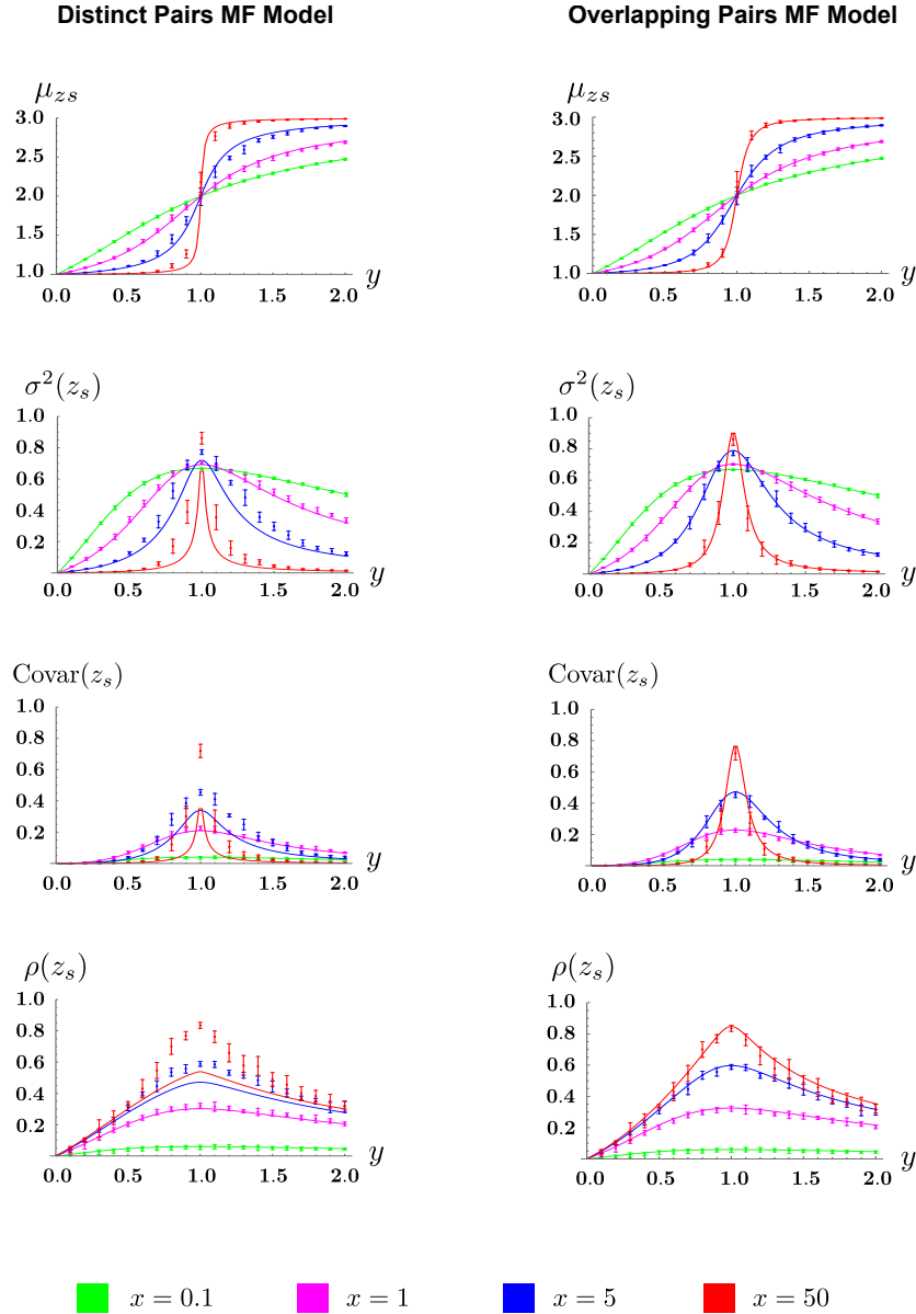
Figure 9: The OPMF model accurately predicts associations between neighbouring CpGs. Predictions of the means ( \mu_{z_s} ), variances ( \sigma^2(z_s) ), covariances ( \text{Covar}(z_s) ) and correlations ( \rho(z_s) ) are plotted against y for the DPMF model (left) and OPMF model (right). For each model, the predictions of the statistics are shown by solid lines (with different colours denoting predictions for different values of x ). The points and error bars correspond to the ground-truth statistics obtained from n = 10 replicate simulations of the full nearest-neighbour model (the mean results obtained from the ten simulations are shown by points, with the error bars denoting the standard error of this estimate across the ten simulations). Note that, since z is determined by x and y , the statistics plotted here are implicit functions of x and y .
