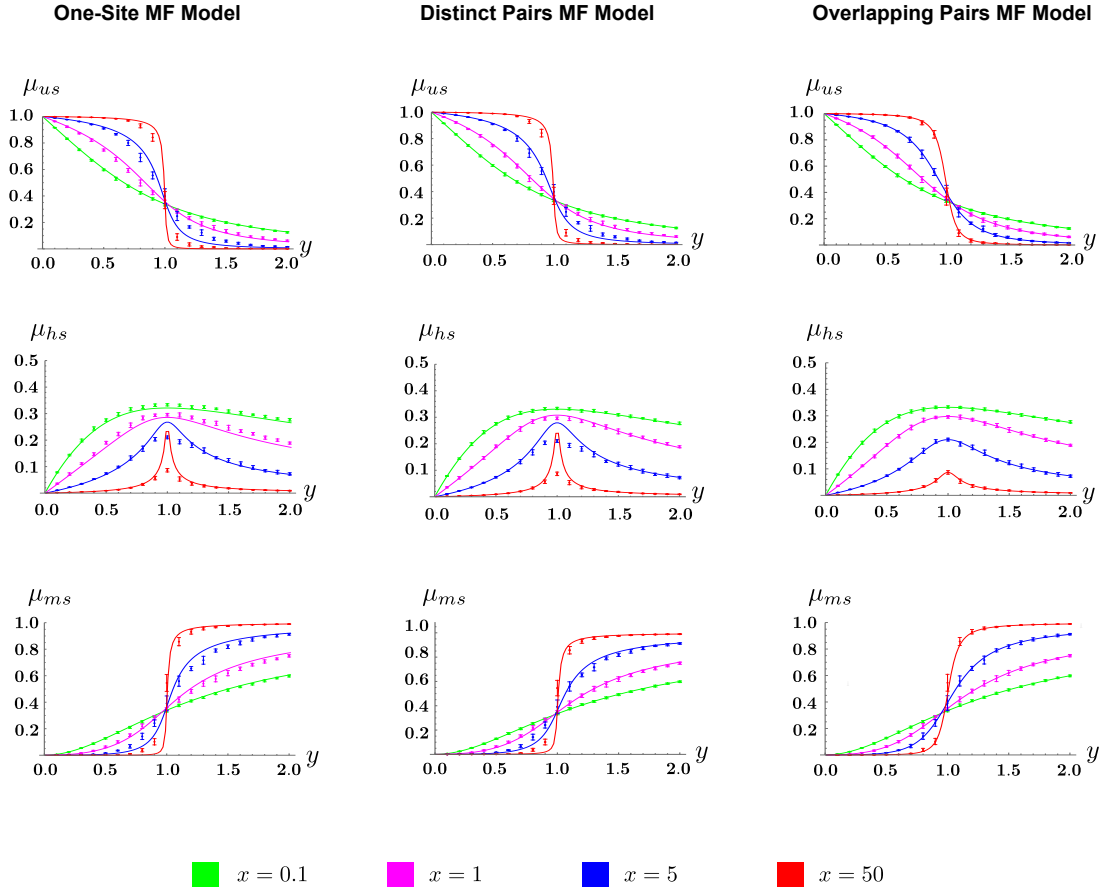
Figure 8: The OPMF model accurately predicts the average behaviour of large-scale methylation patterns. The mean u , h and m levels are plotted against the methylation strength y for the different models and collaboration strengths, x (left: one-site MF model, middle: DPMF model and right: OPMF model). For each model, the predictions of the means are shown by solid lines (with different colours denoting predictions for different values of x ). The points and error bars correspond to the ground-truth means obtained from n = 10 replicate simulations of the full nearest-neighbour model (the mean results obtained from the ten simulations are shown by points with error bars denoting the standard error in this estimate across the ten simulations).
