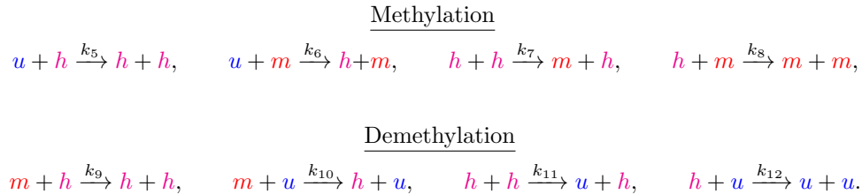
Figure 1: System of reactions under consideration. Here u , h and m represent unmethylated, hemimethylated and methylated CpGs, respectively. Non-collaborative reactions involve only one CpG, while collaborative reactions involve two CpGs. For each collaborative reaction, the second reactant (the mediator—see text) recruits an enzyme that changes the methylation state of the first reactant (the target). For example, the reaction u + h \rightarrow h + h involves a hemimethylated CpG at one site recruiting a methylase enzyme which changes the state of a CpG at another site from unmethylated to hemimethylated. Reaction rates are k_i , i = \{1, \dots, 12\} . Note that only one CpG site changes methylation state during each reaction.
