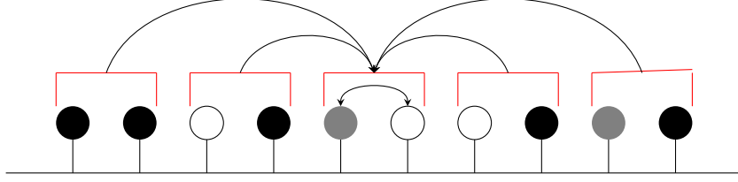
Figure 6: Schematic of the distinct pairs MF model. The two CpGs within a pair can interact directly with each other and the pair is also influenced by the mean state of pairs in the system. In the figure, the uh pair can change state due to interactions between the u and h within the pair, and due to the mean state of pairs in the system.
