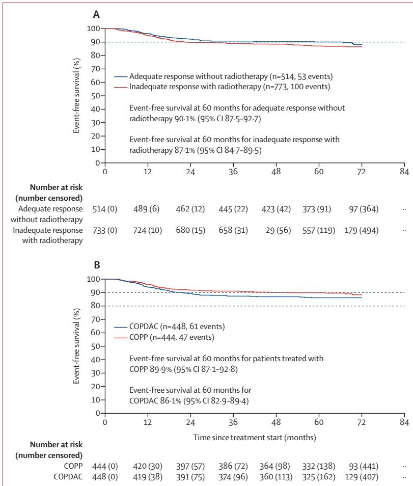
Figure 2: Event-free survival of patients in the per-protocol group in the titration trial and the embedded randomised trial
