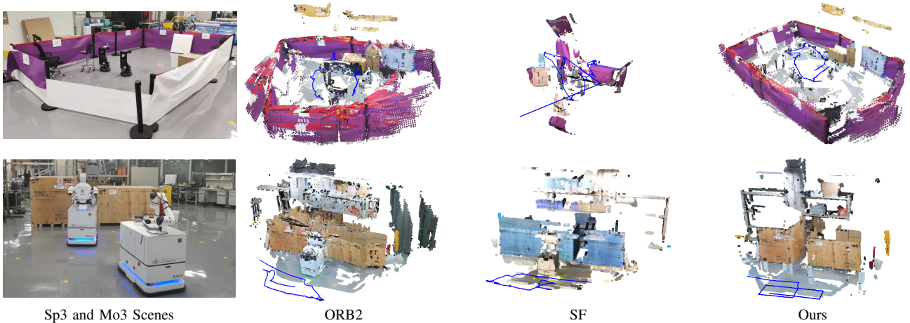
Fig. 7: Dynamic scene mapping results. Top, Sp3 scene. Bottom, Mo3 scene. In both, a robot performs SLAM, another as a dynamic obstacle. The ORB2 and SF methods fail, while our approach build accurate environment maps. The estimated camera trajectories are displayed in blue.
