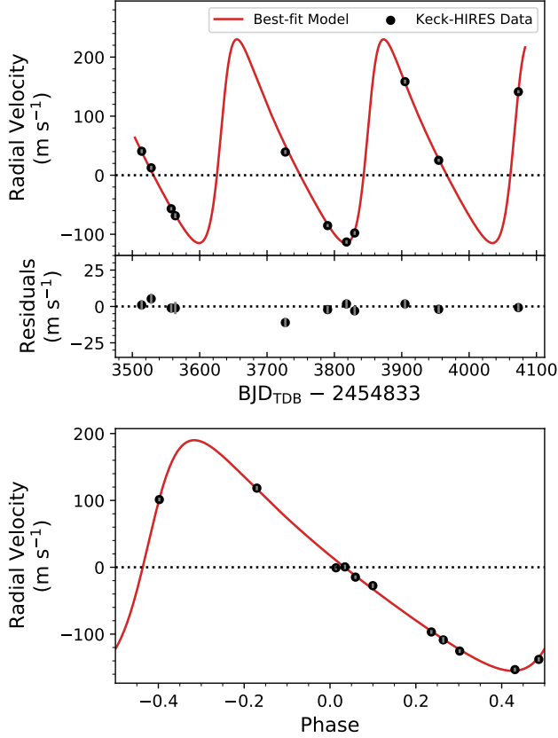
Figure 6. RV measurements of Kepler-1514 from Keck-HIRES. The top panel is the time series data and the bottom panel shows the data phase folded on the best-fit ephemeris using the time of conjunction ( T_C ) as the reference point. Error bars are small but are shown in gray in each panel.
