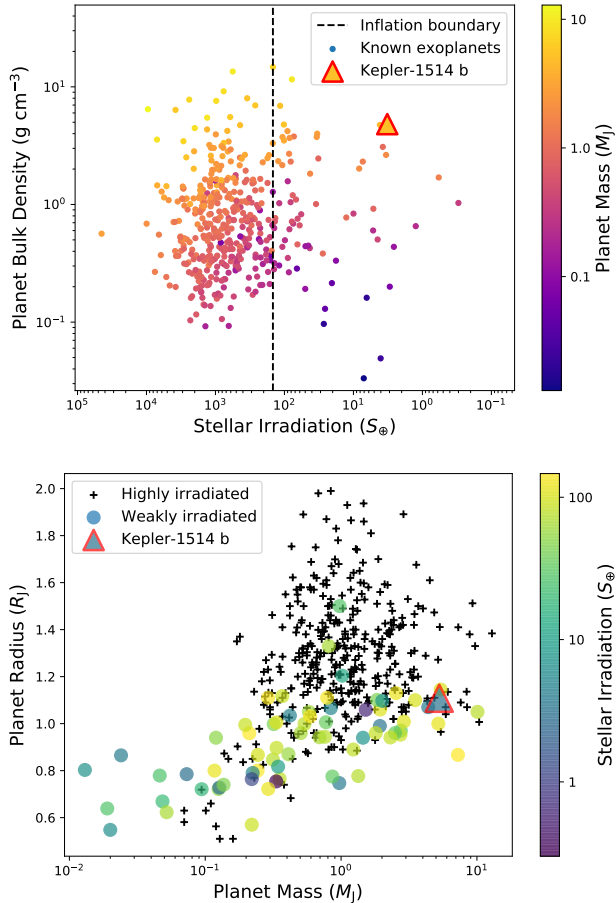
Figure 8. All confirmed giant ( R_p > 0.5 R_J ) exoplanets (from the NASA Exoplanet Archive; accessed 2020 July 9) for which stellar irradiation was either given or could be calculated and planet mass and radius were known to at least 50% precision. Top: of those planets with stellar irradiation below the empirical inflation boundary (Miller & Fortney 2011; Demory & Seager 2011), Kepler-1514 b ranks in the 95th percentile in bulk density. The spread in density is due to the spread in mass, since most of these weakly irradiated giant planets are roughly the same size. Bottom: the inflation boundary from the top panel separates weakly and highly irradiated planets. The combination of high mass and low irradiation for Kepler-1514 b places it among a small group of giant planets that are useful for testing models of giant planet interior structure.
