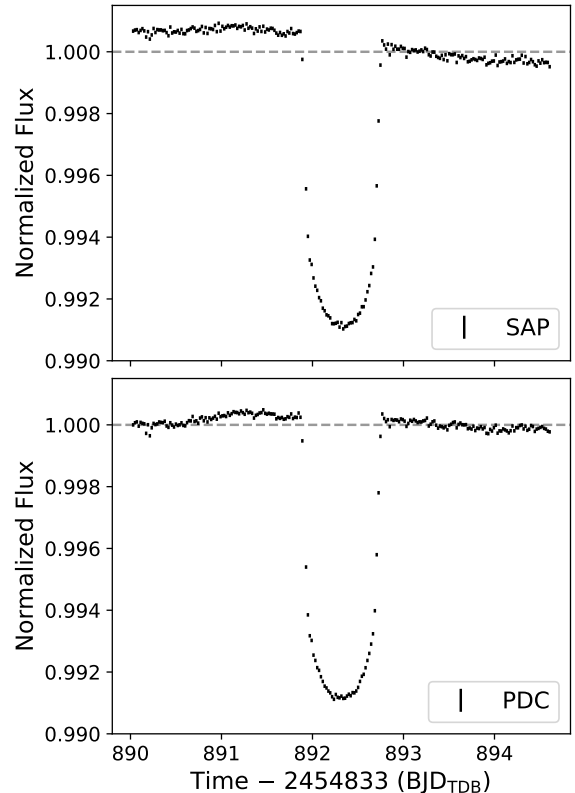
Figure 1. Median-normalized, transit light curve of Kepler-1514 b from Quarter 9 using Kepler SAP (top) and PDC (bottom) data products. We explore whether the variability that is present in these light curves could account for the TTVs, T \delta Vs, and TDVs measured by Holczer et al. (2016) in our modeling of this system.
