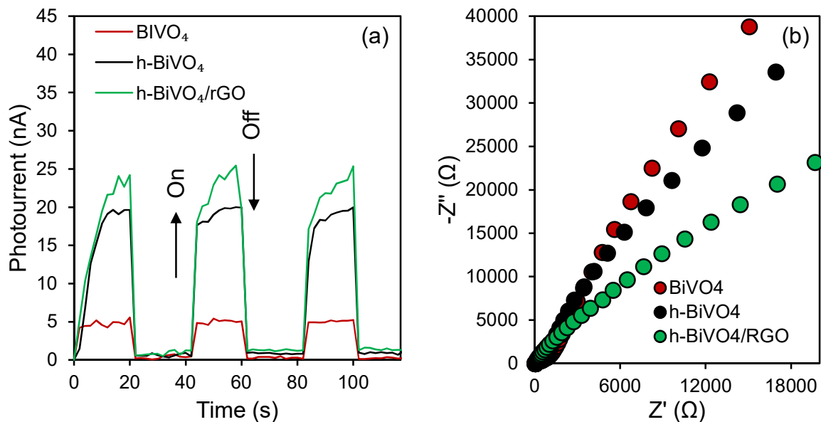
Figure 9. (a) Transient photocurrent signals, and (b) electrochemical impedance spectroscopy for \text{BiVO}_4 , \text{h-BiVO}_4 and \text{h-BiVO}_4/\text{RGO} under visible light illumination ( \lambda > 420\text{nm} ) using a 200 W Hg-Xe arc lamp and 0.5 M \text{Na}_2\text{SO}_4 electrolyte.
