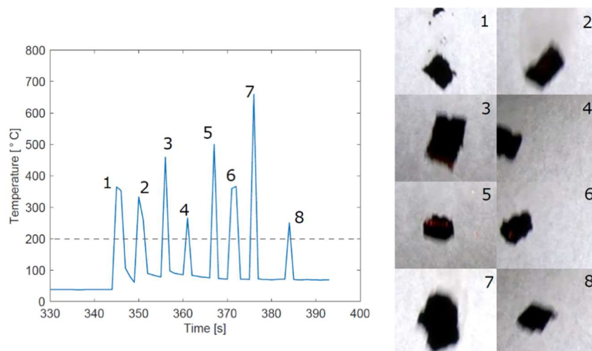
Figure 7 Example showing results from the combined use of the visual and IR camera. Maximum temperature recorded by the IR camera within 1-second time window and images from the visual footage showing the related firebrands. The dashed line indicates the threshold discriminating between reacting (hot) and not reacting (cold) firebrands.
