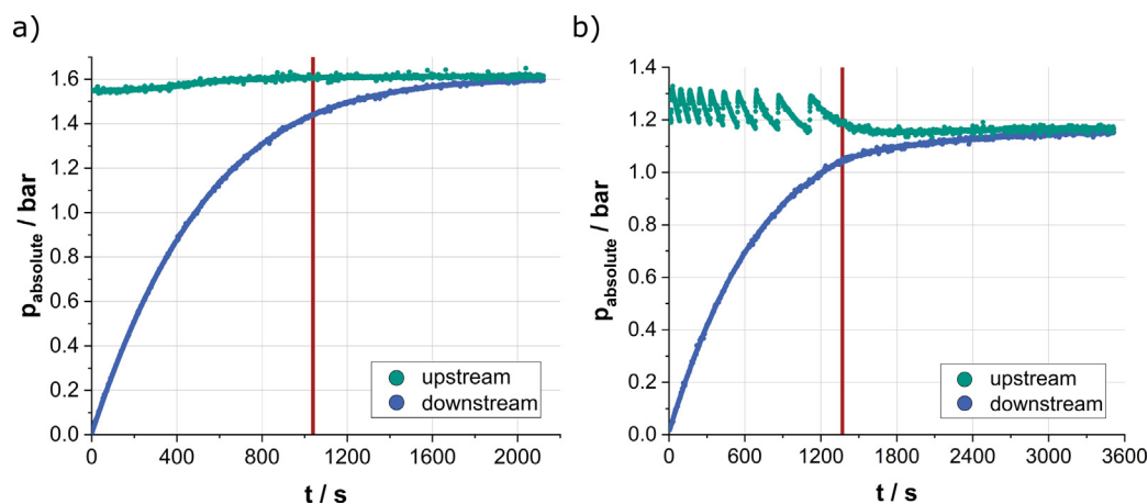
Fig. 9. Temporal evolution of up- and downstream pressure during permeance experiments with sample gasses (a) H 2 or (b) O 2 ; time limit until which the data is considered for evaluation marked by a red line.
