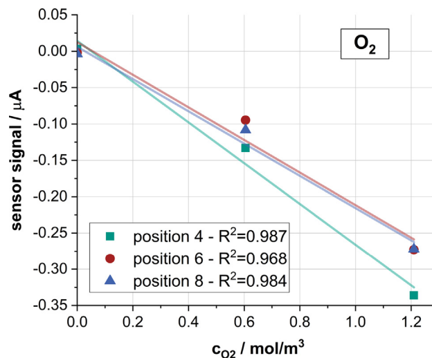
Fig. A1. O_2 calibration curves of the electrochemical sensors mounted in positions 4, 6 and 8.
