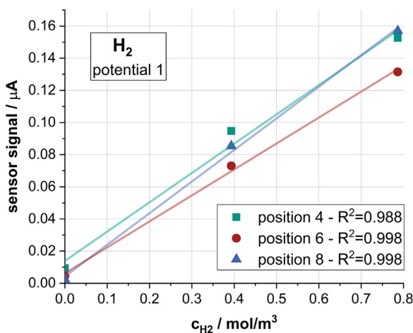
Fig. A2. H_2 calibration curves of the electrochemical sensors mounted in positions 4, 6 and 8 for two different potentials, (a) and (b).
