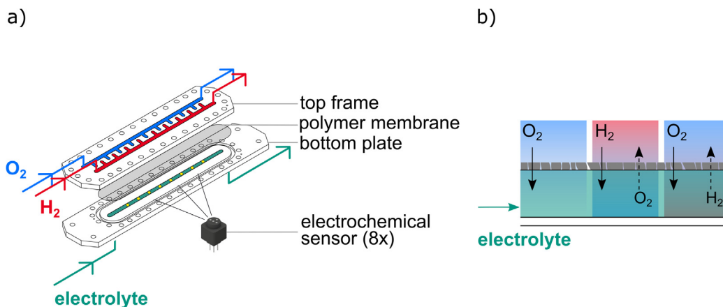
Fig. 1. (a) Schematics of the membrane reactor designed for the direct synthesis of H_2O_2 in a microstructured membrane reactor, adapted from (Urban et al., 2021). (b) Schematics of the problem of counter-diffusion.
