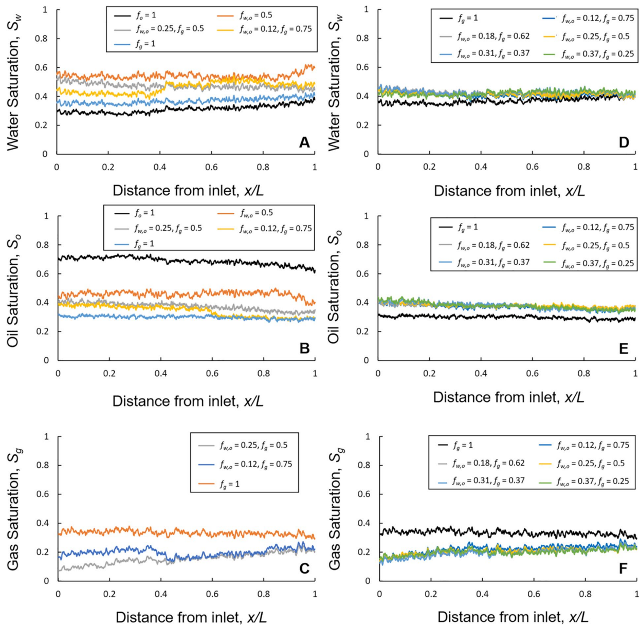
Figure 13. Fluid saturation profiles of (a) water, (b) oil, and (c) gas during increasing gas fractional flow, decreasing oil and water fractional flows, and of (d) water, (e) oil, and (f) gas during decreasing gas fractional flow, increasing oil and water, plotted along the length of the whole sample. Fluid saturations in the macro-pores only are considered. Note that the saturation profiles are approximately constant with distance indicating that there is no noticeable capillary end effect. Gas, oil, and water fractional flows ( f_g and f_{w,o} ) are stated.
