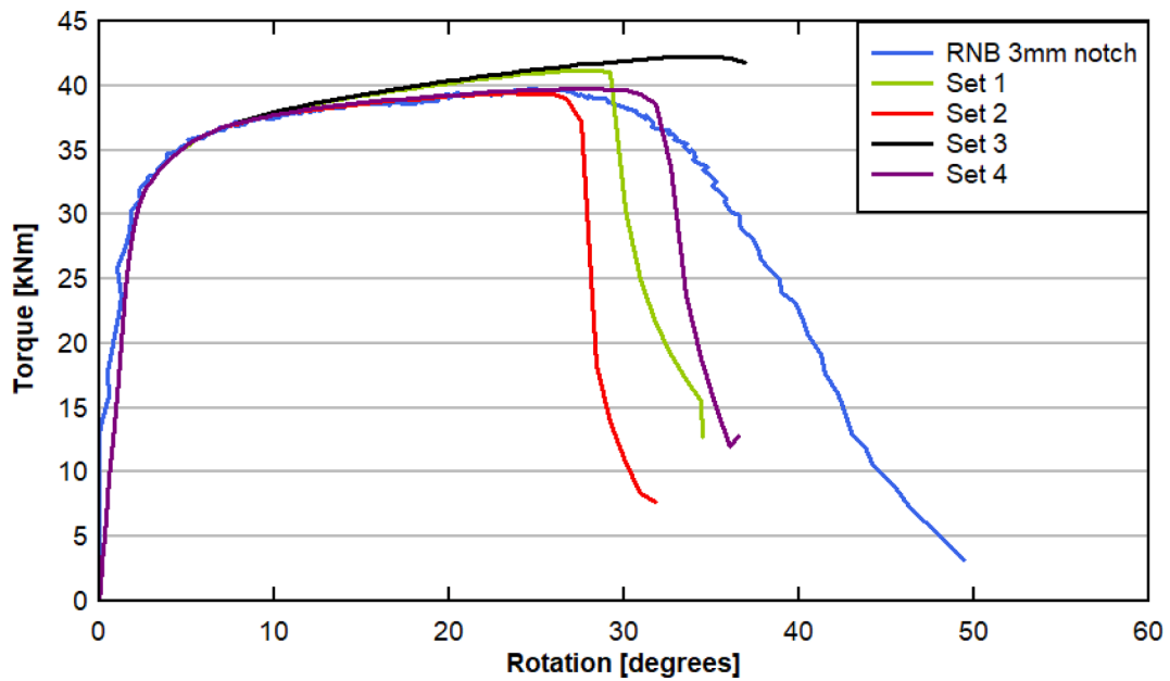
Fig. B8. RNB3 torsion simulation response.
