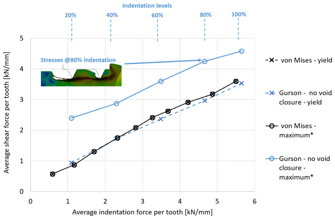
Fig. 21. Connection strength vs indentation force for the two-teeth model.
