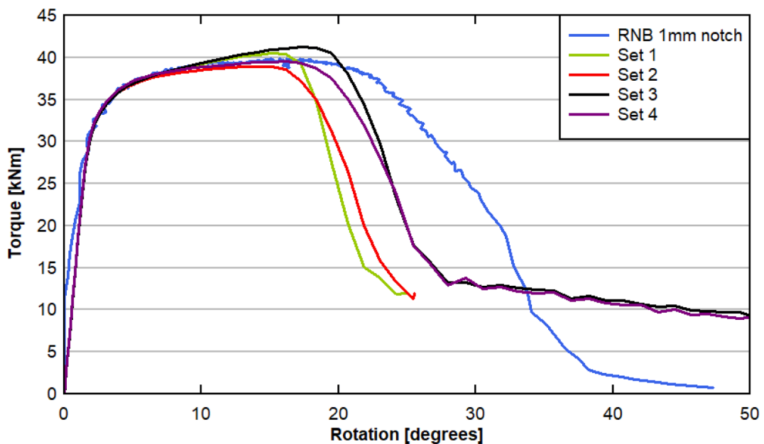
Fig. B7. RNB1 torsion simulation response.
