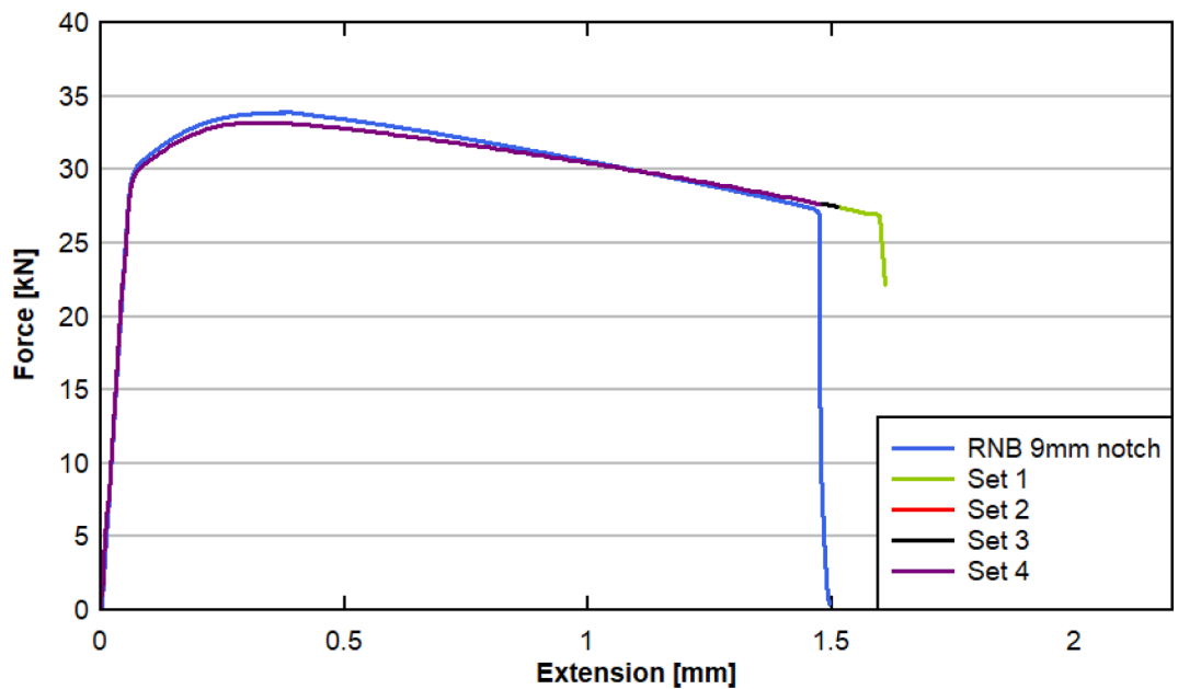
Fig. B5. RNB9 tension simulation force-displacement response.
