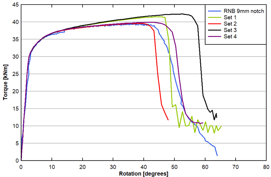
Fig. B9. RNB9 torsion simulation response.
