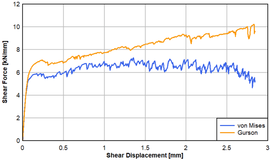
Fig. 15. Shear force vs shear displacement response of setting simulation with extended Gurson and von Mises models. The extended GTN model uses the Set 4 calibrated parameters and the von Mises model uses the Low HC curve.
