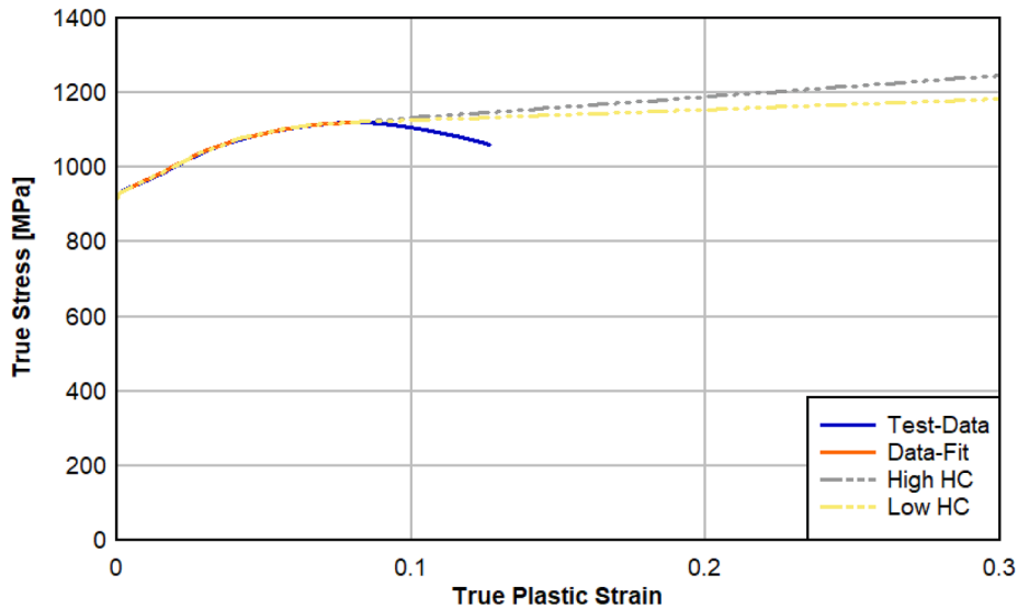
Fig. 9. Extrapolated Hardening Curves.
