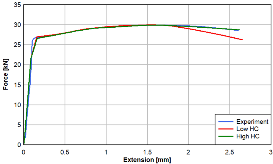
Fig. 10. RDB comparison of hardening curves.
