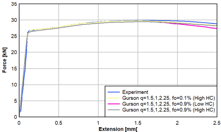
Fig. 11. Force displacement response of RDB simulations.
