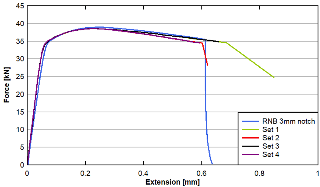
Fig. B4. RNB3 tension simulation force-displacement response.
