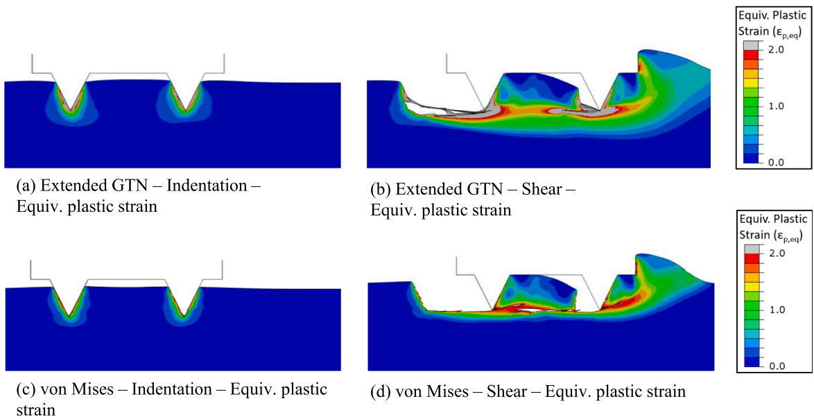
Fig. 14. Equivalent Plastic Strains with: (a) extended GTN model after 80% indentation, (b) extended GTN model after shear, (c) von Mises model after 80% indentation and (d) von Mises model after shear. The extended GTN model uses the Set 4 calibrated parameters and the von Mises model uses the Low HC curve.
