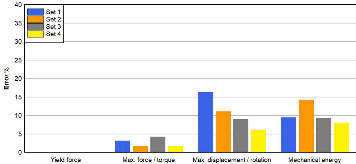
Fig. 12. Performance evaluation of calibrated parameter sets.
