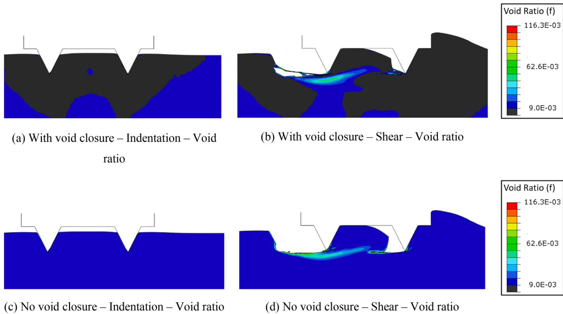
Fig. 16. Void ratio with: (a) extended GTN model after 80% indentation with possibility of void closure, (b) extended GTN model after shear with possibility of void closure, (c) extended GTN model after 80% indentation with no void closure allowed, (d) extended GTN model after shear with no void closure allowed. The extended GTN model uses the Set 4 calibrated parameters and the von Mises model uses the Low HC curve.
