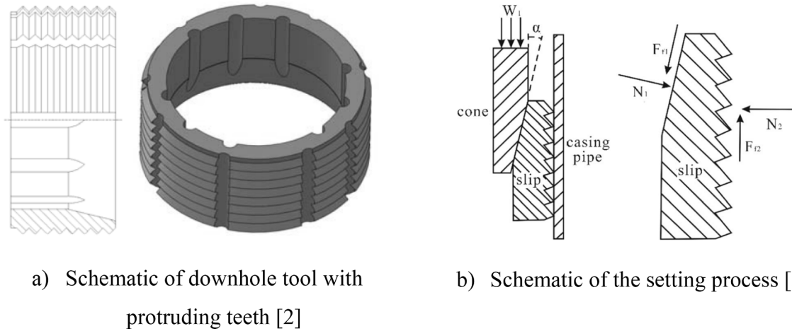
Fig. 1. Setting process schematic from [2] & [3]. The schematic shows the tool setting on casing pipe, which is achieved by indentation of slips into the casing wall.
