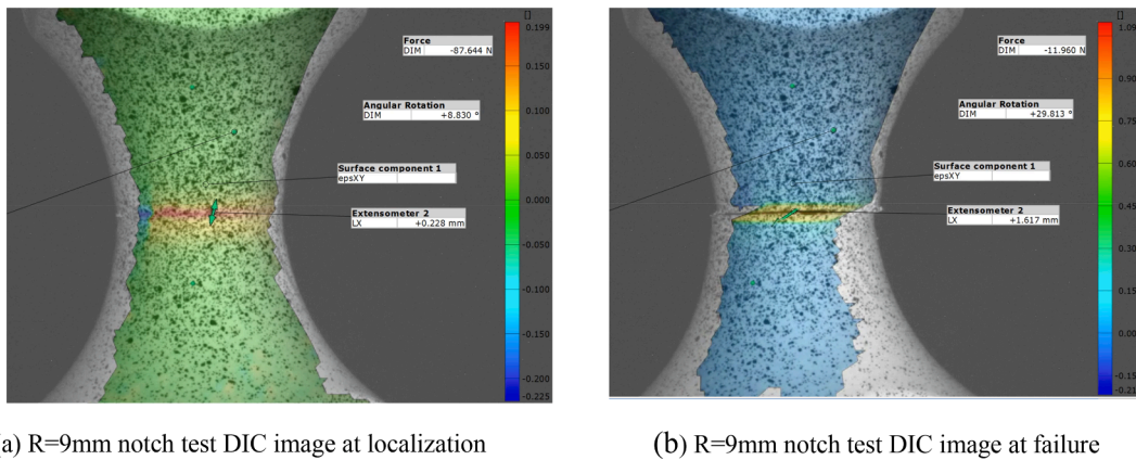
Fig. 8. RNB R = 9 mm notch test DIC images at (a) localization and (b) failure.
