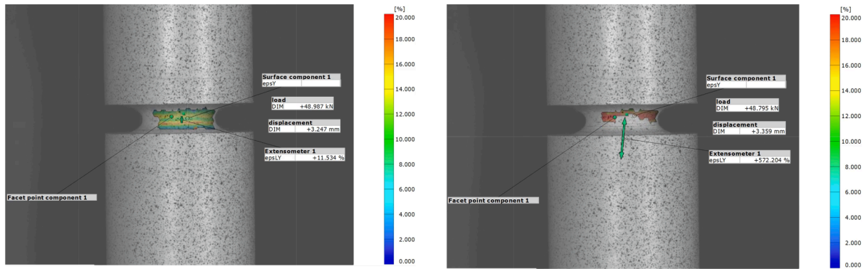
(a) R=1mm notch test DIC image at localization
