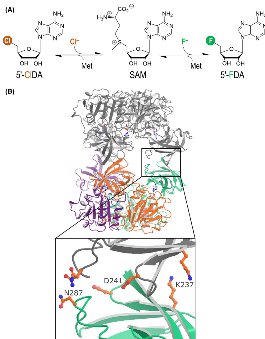
Fig. 1. A. Reactions catalysed by the fluorinase enzyme. Abbreviations are as follows: Cl - , chloride ion; F - , fluoride ion; SAM, S -adenosyl- L -methionine; Met, L -methionine; 5'-CIDA, 5'-chloro-5'-deoxyadenosine; and 5'-FDA, 5'-fluoro-5'-deoxyadenosine. B. A 3D model of the FIA fluorinase enzyme from Streptomyces sp. strain MA37. The amino acid residues sitting at the trimer-trimer interface, critical for the formation of the hexameric form, are highlighted in the inset.
