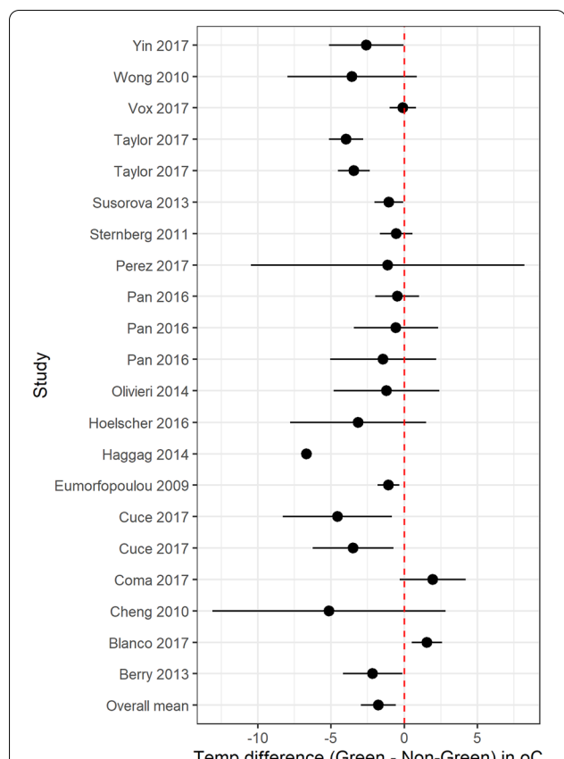
Fig. 17 Forest plot for effect of green walls on surface temperature. The Y-axis shows study first author and date. The X-axis shows the difference in ST between green walls and non-green wall surfaces. Some studies are associated with more than one effects size if the data were presented for different seasons or times of day. For full citation and meta-data for each study see Additional files 1 and 2 for details of data sources
