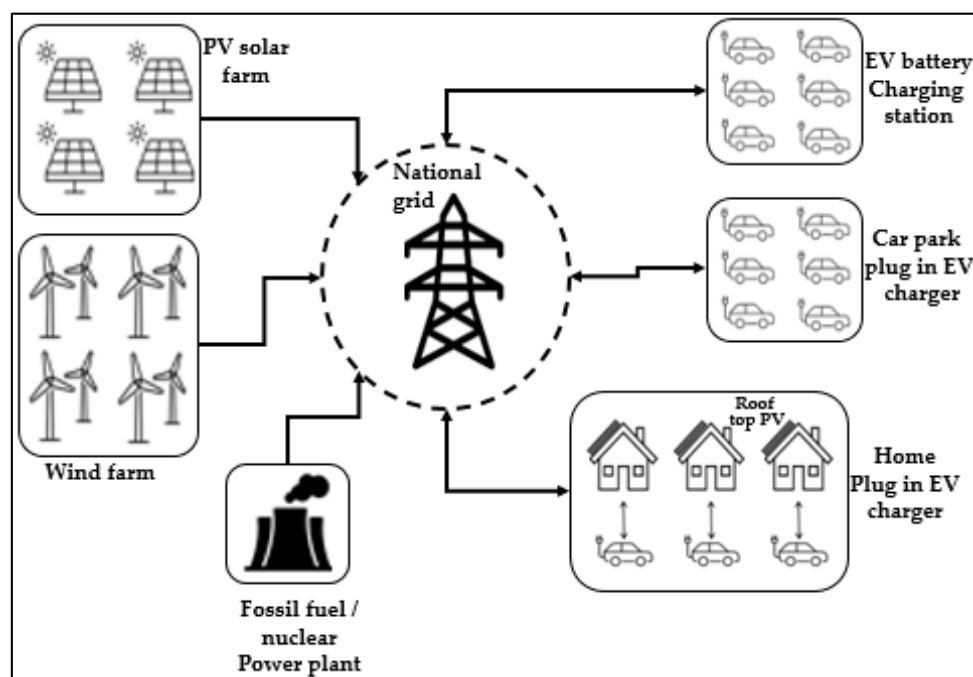
Figure 12. Schematic layout of V2G architecture.
