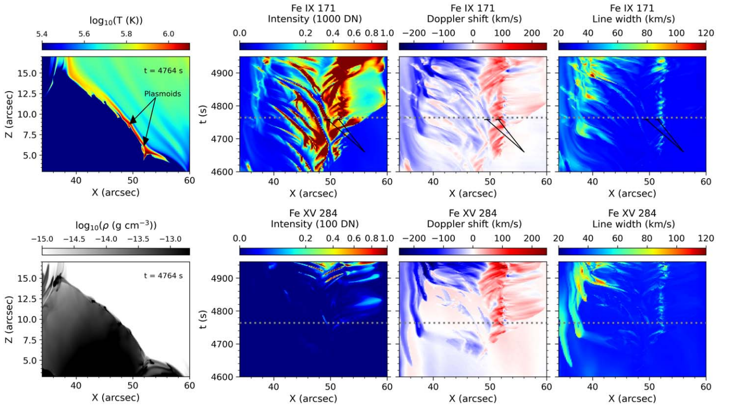
Figure 15. Formation and ejection of multiple plasmoids within an elongated current sheet in the Bifrost simulation B_{\text{npdms03}} (see Table 1 and Appendix A). The left column shows the temperature (top) and mass density (bottom) at time t = 4764 s of the run. The panels on the right contain X - t maps (computed for an LOS direction parallel to the z -axis) of the MUSE Fe IX 171 Å (top) and Fe XV 284 Å (bottom) moments, namely, the intensity, Doppler shift, and line width. The horizontal dotted line in these panels corresponds to the time shown in the temperature and density panels. An animation of the figure is also available showing the evolution of the temperature and density between t = 4602 s and t = 4946 s. The real-time duration of the animation is 7 s.
