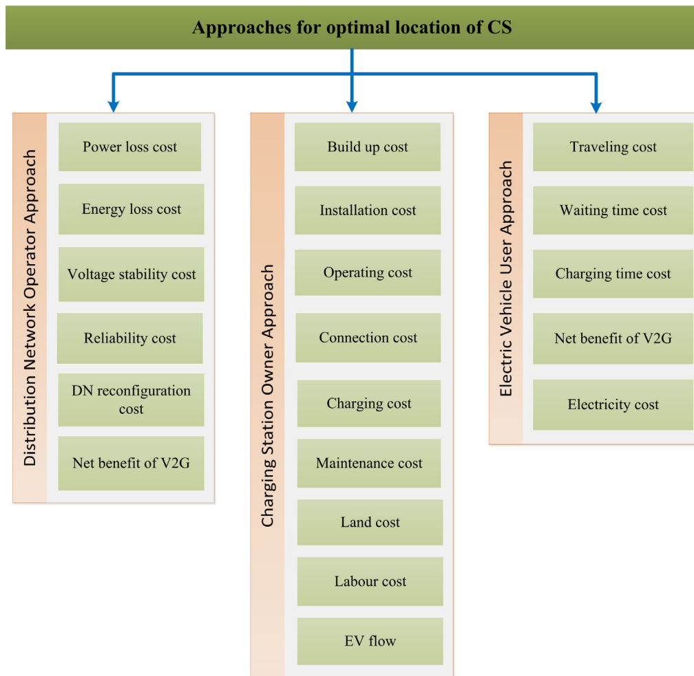
Fig. 3. Approaches of problem formulation for placement of EVCS.
