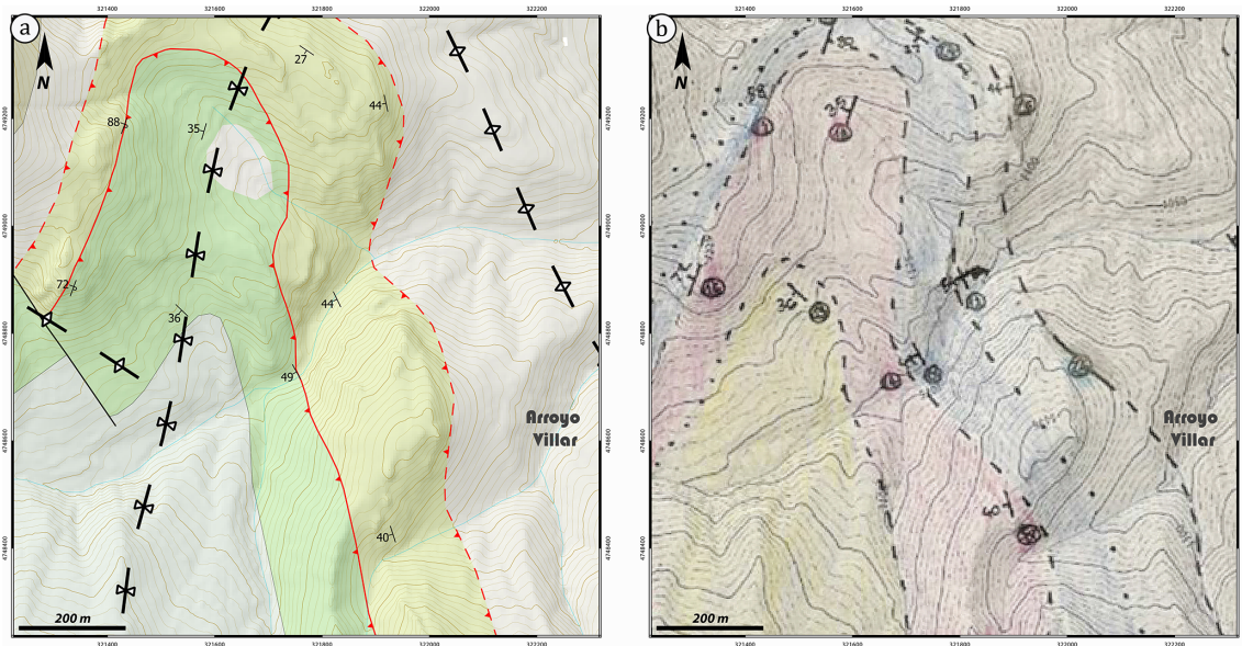
Figure 6. Detail of the geological map of the Esla Nappe immediately west from the locality of La Velilla de Valdoré (see Fig. 1b for the location). (a) Modified version of the continuous digital geological map of Spain (GEODE) from the Spanish Geological Survey (modified from Merino-Tomé et al., 2014). Bedding data are the same as those provided to the students in the Esla Mapping Project. (b) Geological map produced by one of the students as a result of the Esla Mapping Project. Note that the cross section shown in Fig. 3b was not drawn through the syncline shown in this map but through the more eastern Pardominos Anticline (axial trace shown on the NE corner of a).
