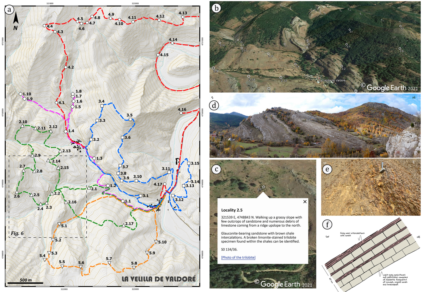
Figure 2. Outline of different elements of the Esla Mapping Project. (a) Daily itineraries of realistic walking distance with a number of stops along the way. The XY notation refers to the day (X) and the stop (Y). Map derived from digital elevation model provided by IGN (National Geographic Institute of Spain). See Fig. 1a for the location. (b) Tilted view of the northern part of the mapping area looking north with the stops shown as white symbols (© Google Earth 2021). Based on the information contained on each of the stops, students coloured the pins accordingly. (c) Example of data provided to the students at one of the stops. The photo of the trilobite is accessed by a link to an image stored in the GitHub repository, opened within Google Earth (© Google Earth 2021). (d) Panoramic view provided at stop 3.13 looking west: students were asked to inspect it and draw an annotated field sketch. (e) Outcrop photograph provided at stop 4.3 to familiarise the students with the provided rock description. (f) Outcrop sketch provided as data to the students at stop 5.1.
