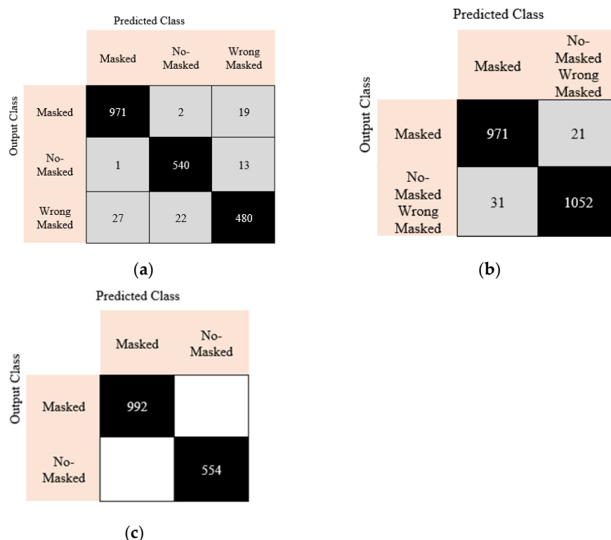
Figure 6. Confusion matrices resulting from training and testing the model with the three different cases: (a) Case 1, (b) Case 2, and (c) Case 3.
