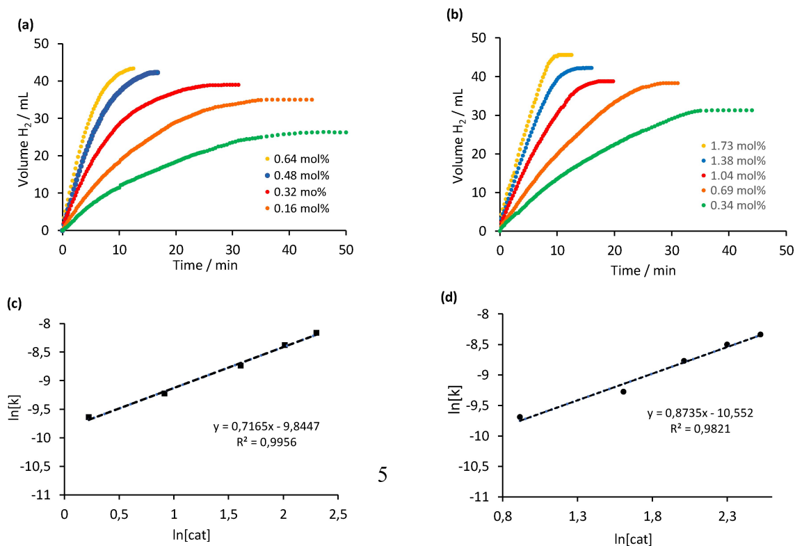
Figure 7. (a) and (b) Plots of volume of hydrogen vs time for the hydrolysis of 2 mL of 0.27 M \text{NaBH}_4 at 35 °C catalyzed by various concentrations of 3a and 3b , respectively; (c) and (d) plots of hydrogen generation rate vs concentration of catalyst in logarithmic scale for 3a and 3b , respectively. Volumes measured are an average of three runs.
