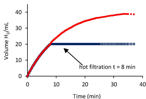
Figure 13. Hot filtration test for the hydrolysis of NaBH 4 using 0.32 mol% 3 a showing that turnover has been completely quenched after filtration at t=8 \text{ min} . Red line – reaction in the presence of catalyst; blue line reaction catalyzed by 3 a and filtered to remove catalysts after 8 min.
