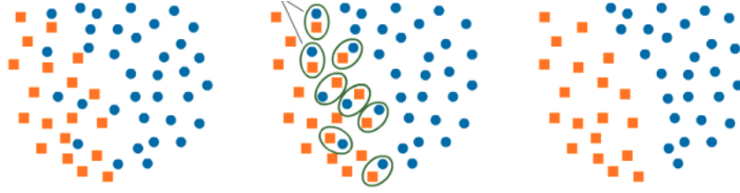
Figure 4.3: The balanced class distribution by NearMiss
