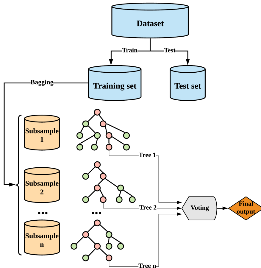
Figure 2.8: The structure of random forest
