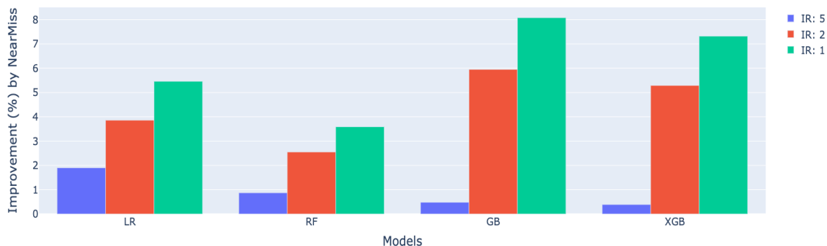
Figure 4.9: AUC improvement of classification models by undersampling method (NearMiss) against LR on original dataset (IR=13.9)
