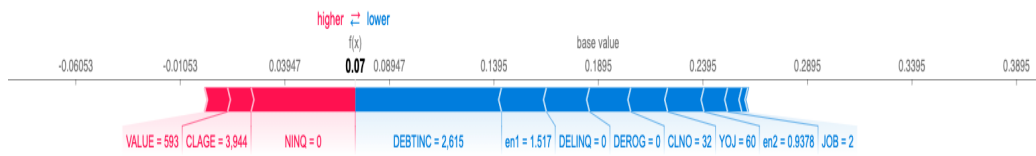
Figure 5.11: SHAP value plot for individual sample predicted by RF of NOTE
