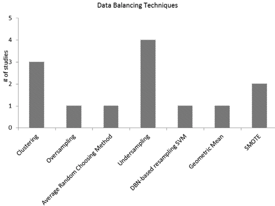
Figure 1.1: The number of studies for balancing datasets in credit scoring models (Dastile et al., 2020)
