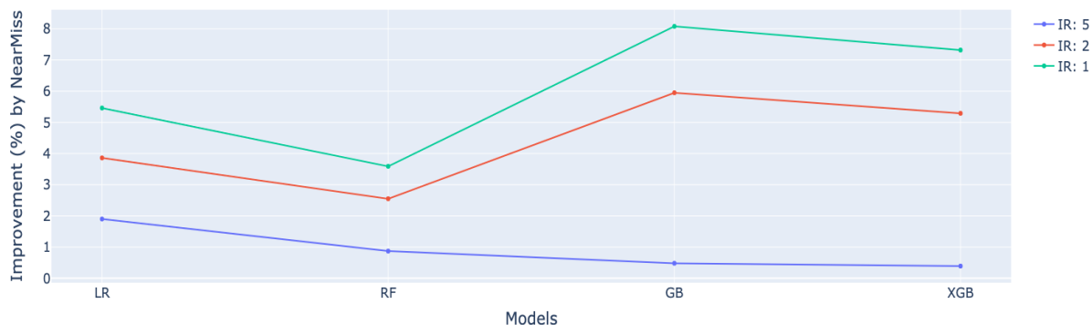
Figure 4.12: AUC improvement of classification models by undersampling method (NearMiss) against LR on original dataset (IR=13.9)
