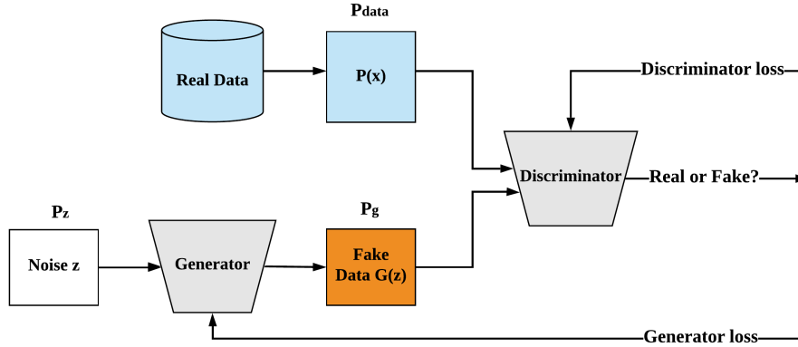
Figure 5.3: The structure of GAN-based generation for synthetic data
