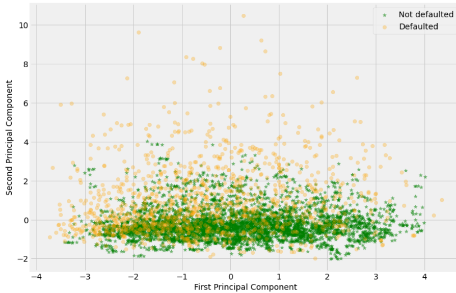
Figure 5.1: The imbalanced class on HE dataset
