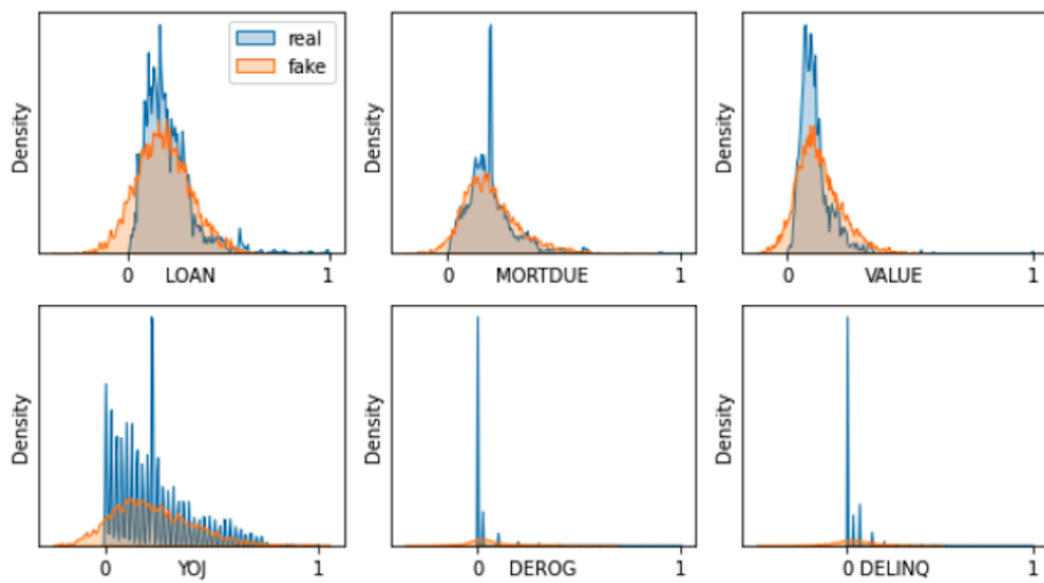
Figure B.1: Comparison between real and generated distribution of numerical features by NOTE on HE dataset
