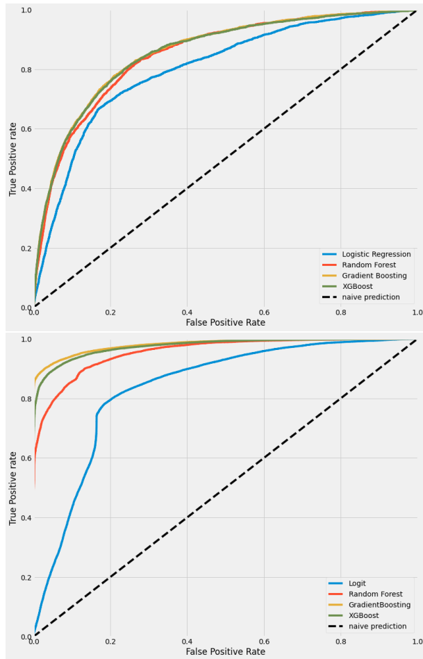
Figure 4.11: The ROC of non-parametric classifier against parametric model on original dataset (above) and balanced dataset (below)
