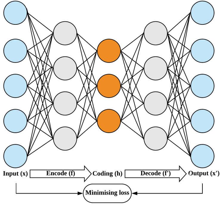
Figure 3.4: The structure of SAE
