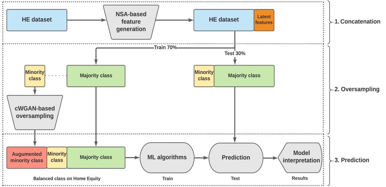
Figure 5.5: The system architecture of NOTE
