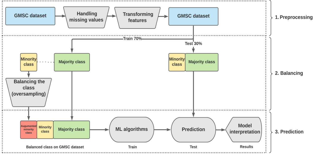
Figure 4.6: The system architecture
