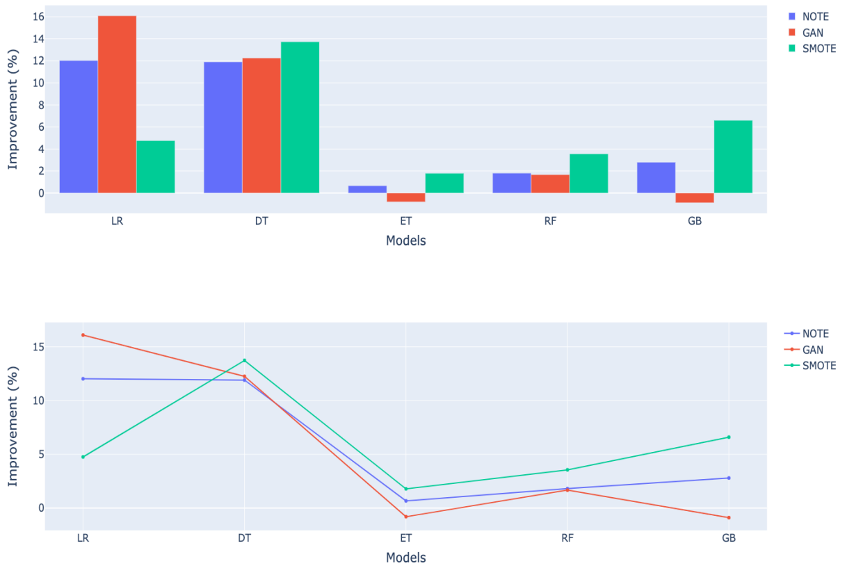
Figure 5.8: AUC improvement of classification models by oversampling methods against non-resampling
