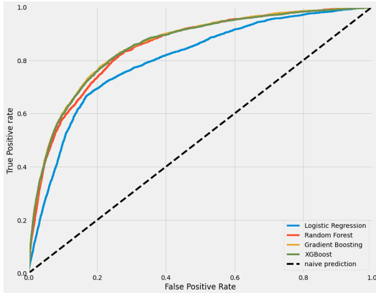
Figure 2.3: An example of ROC curve
