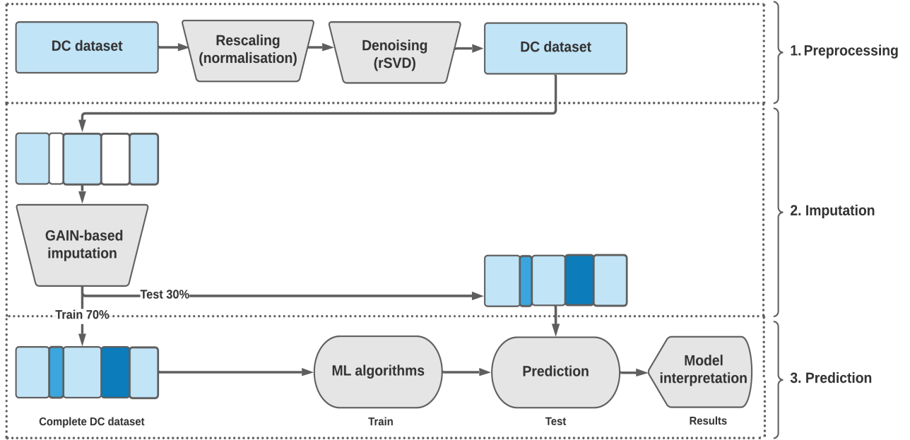
Figure 6.4: The system architecture of DITE
