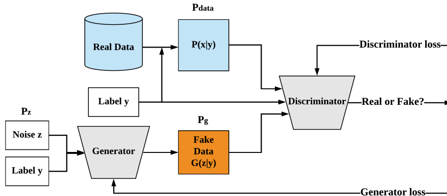
Figure 5.4: The structure of cGAN-based generation for synthetic data
