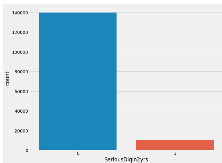
Figure 4.2: The imbalanced class on GMSC dataset, where 0 means not defaulted (good credit) and 1 means defaulted (bad credit)
