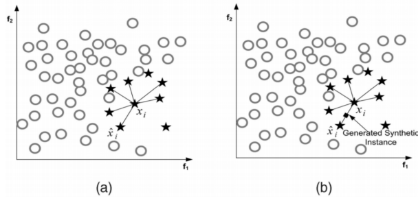
Figure 4.4: The synthetic sample generated by SMOTE
