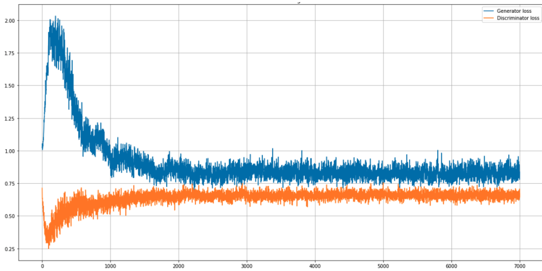
Figure B.3: The loss of generator and discriminator in GAN on HE dataset
