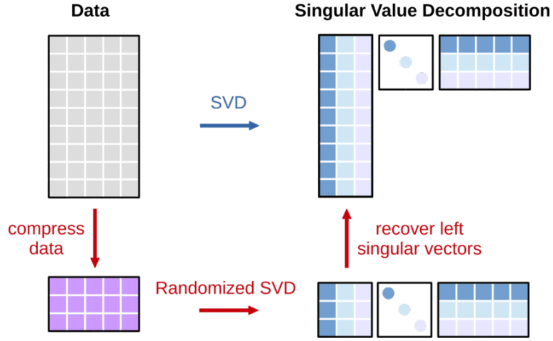
Figure 6.2: The conceptual architecture of rSVD
