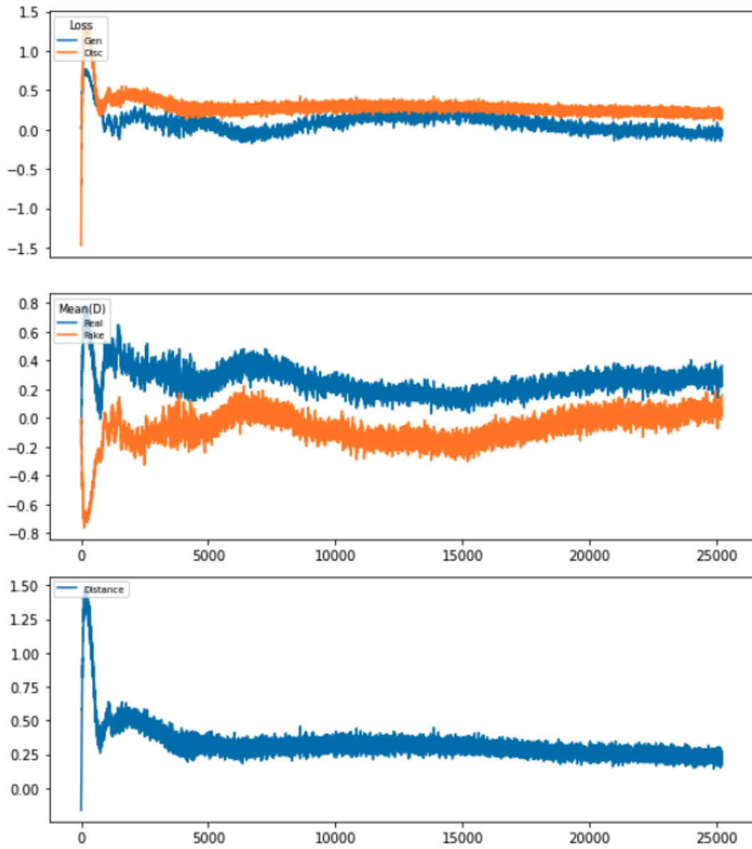
Figure B.2: The loss of generator and discriminator in NOTE (cWGAN) on HE dataset
