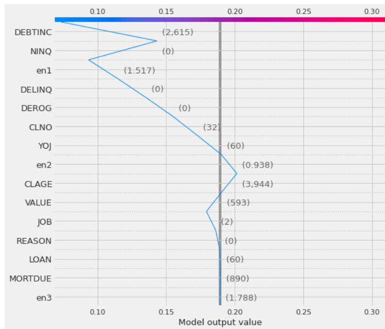
Figure 5.11: SHAP value plot for individual sample predicted by RF of NOTE
