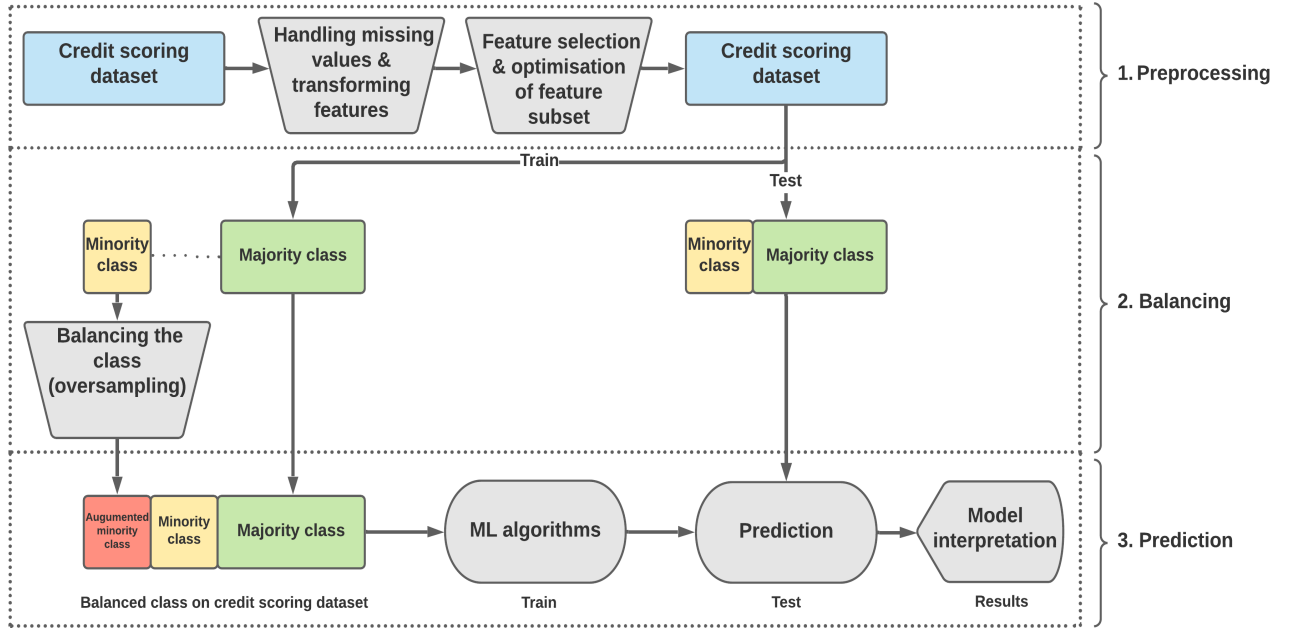
Figure 3.2: The general framework for credit scoring using ML models
