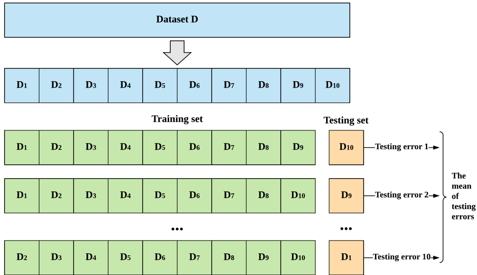
Figure 2.1: 10-fold cross-validation
