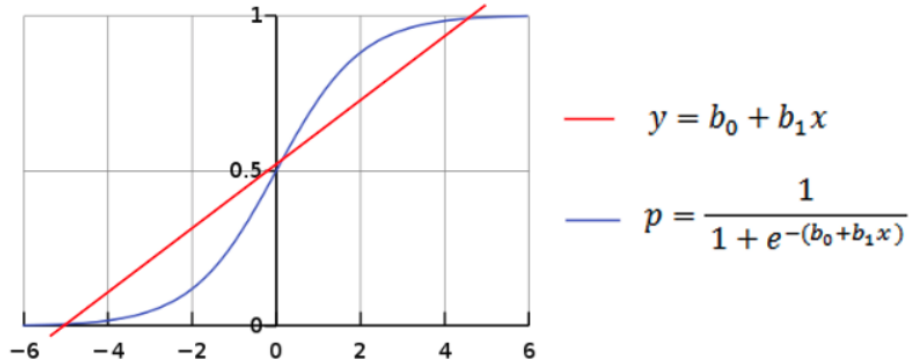
Figure 2.5: Linear model and logistic curve
