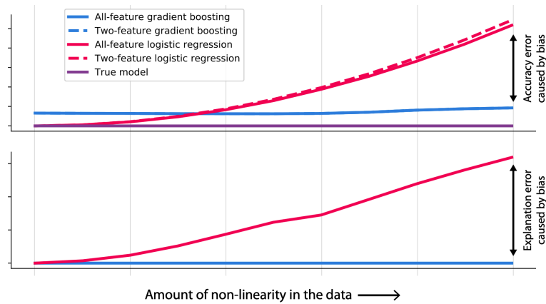
Figure 4.1: Comparison between LR and GB regarding the error of explanation and accuracy (Lundberg et al., 2020)
