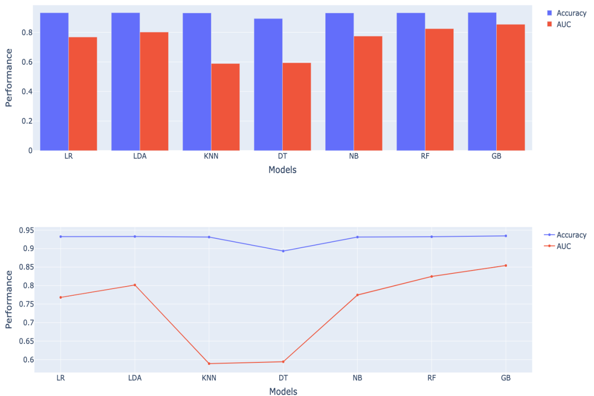
Figure 4.7: The performance comparison for accuracy and AUC between ML models on original dataset
