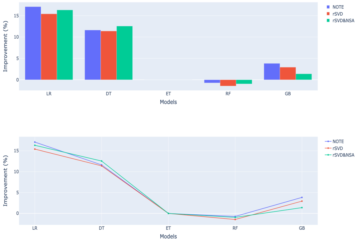
Figure 5.9: AUC improvement of classification models by extracting and denoising methods against benchmarks (Engelmann and Lessmann, 2021), AUC of ET: N/A
