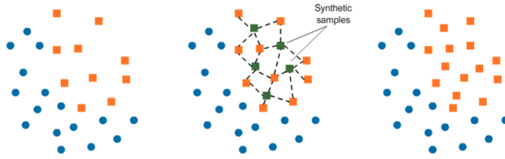
Figure 4.5: The balanced class distribution by SMOTE
