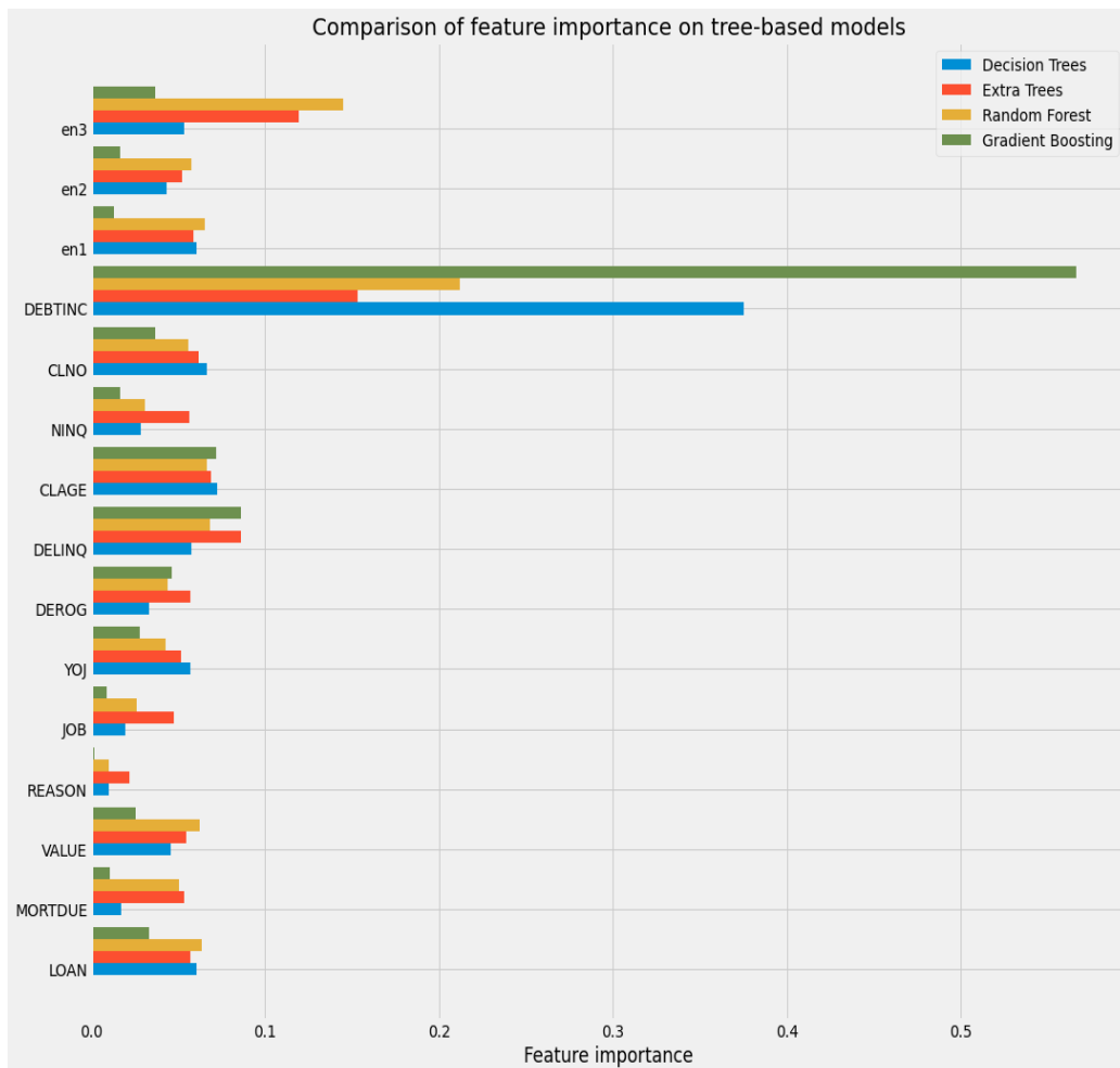
Figure 5.14: Comparison of feature importance on tree-based models of NOTE, where en1, en2 and en3 are latent representation extracting from NSA
