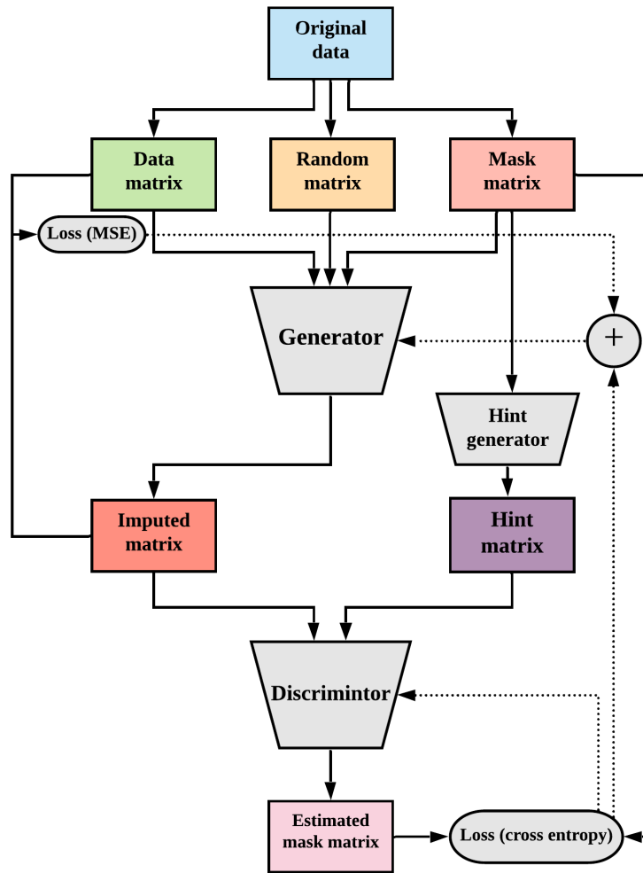
Figure 6.3: The architecture of GAIN
