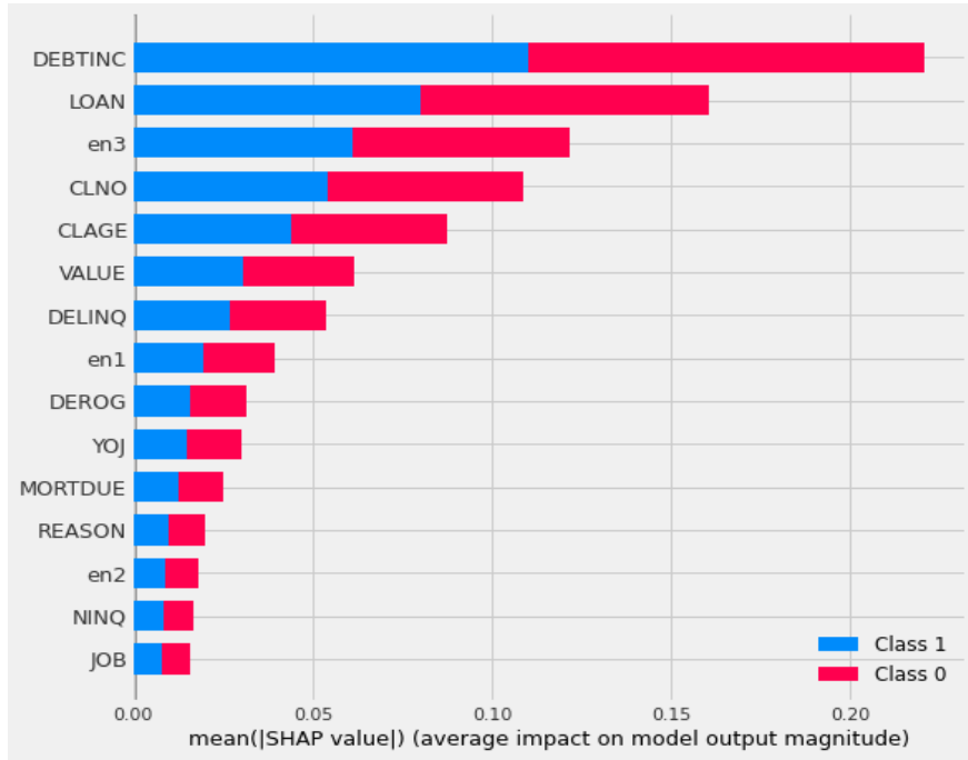
Figure 5.10: Comparison of SHAP feature importance on RF of NOTE, where en1, en2 and en3 are latent representation extracting from NSA
