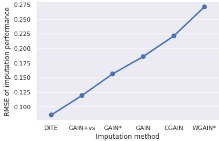
Figure 6.6: RMSE comparison for GAIN-based imputation methods on default credit card with 20% missing data
