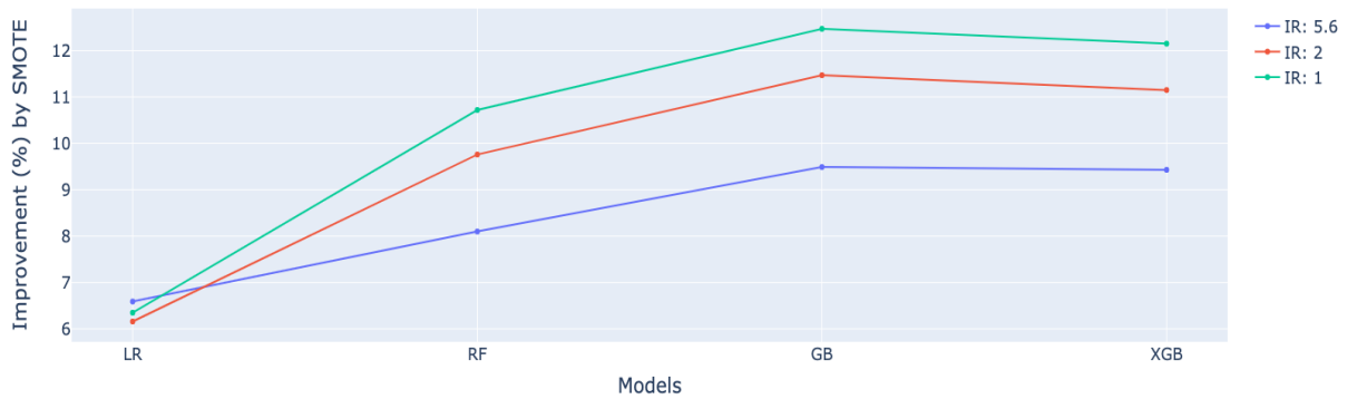
Figure 4.13: AUC improvement of classification models by oversampling method (SMOTE) against LR on original dataset (IR=13.9)
