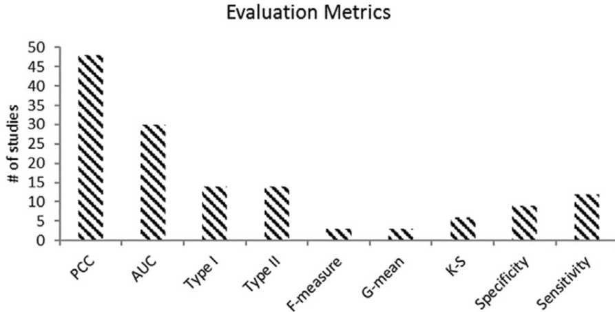
Figure 2.4: The number of studies for evaluating performance in credit scoring models (Dastile et al., 2020)
