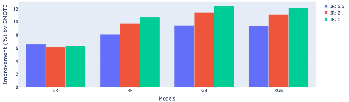
Figure 4.10: AUC improvement of classification models by oversampling method (SMOTE) against LR on original dataset (IR=13.9)
