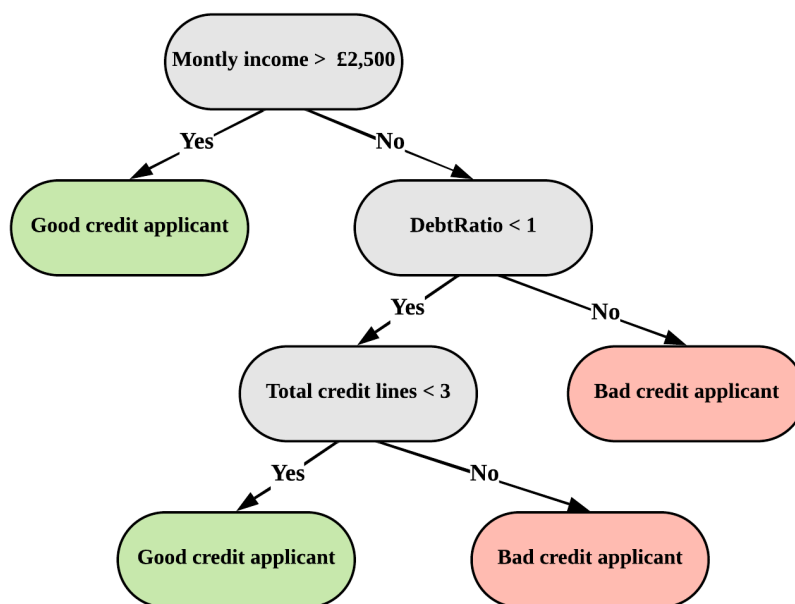
Figure 2.6: A hypothetical example of DT model in credit scoring
