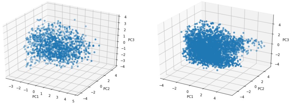
Figure 5.7: PCA of minority class with 1,189 original samples (left) and 3,582 generated samples (right)
