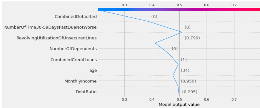
Figure 4.16: SHAP decision plot for individual sample predicted by GB
