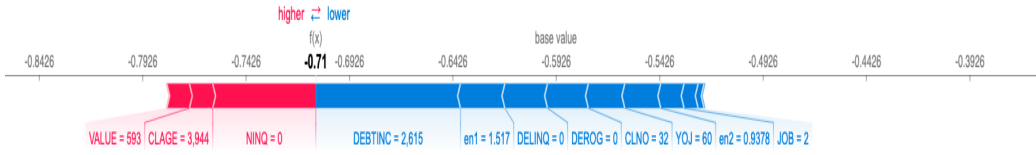
Figure 5.13: SHAP value plot for individual sample predicted by LR of NOTE
