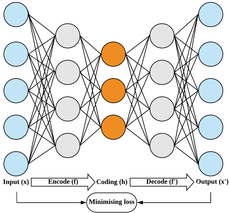
Figure 5.2: The non-parametric stacked autoencoder (NSA), where codings are latent features of original dataset
