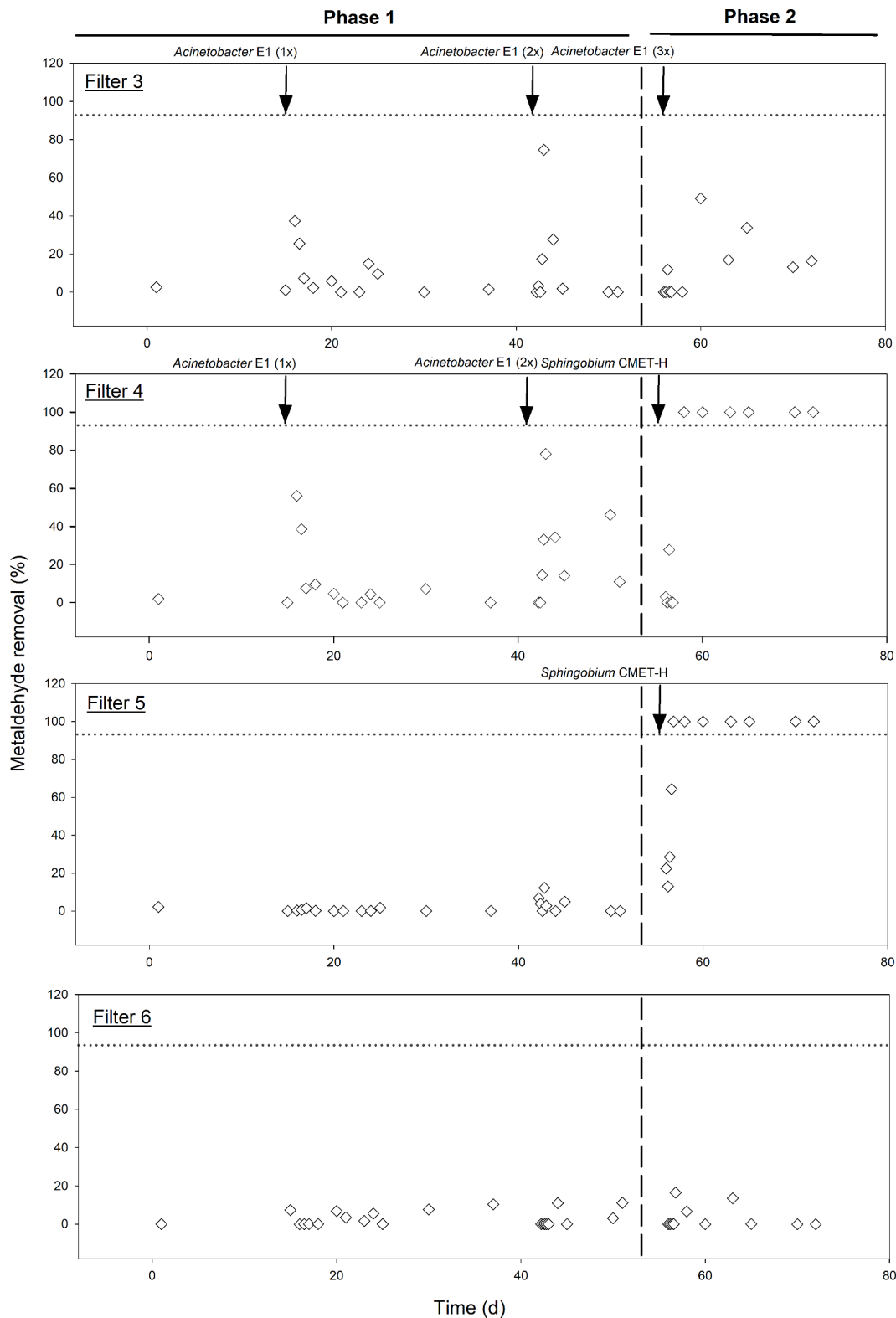
Fig. 2. Percentages of metaldehyde removal calculated as 100 - \{([metaldehyde]_{outlet} - [metaldehyde]_{inlet}) / [metaldehyde]_{inlet}\} \cdot 100 in SSFs with metaldehyde addition (3 to 6). Arrows indicate the inoculation events of bioaugmentation agents. Dotted lines indicate 95% metaldehyde removal.
