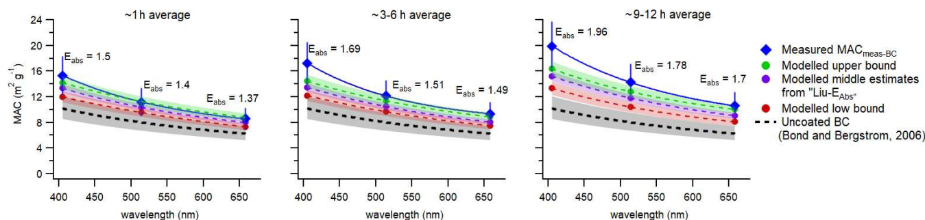
Figure 7. The measured and modelled MAC values at 405, 514 and 658 nm in sampled smoke with different ages, including the measured MAC meas-BC (blue markers), the low (red circle markers) and upper (green circle markers) limits, and approximately middle estimates (purple circle markers, from Liu- E_{Abs} ) of modelled MAC (MAC modelled ). The uncertainties of MAC meas-BC include the instrument uncertainties and the fit errors. The uncertainties of MAC modelled are from the Monte Carlo analysis as in Taylor et al. (2020). The black dashed lines and shaded areas represent the MAC and uncertainties of uncoated BC reported by Bond and Bergstrom (2006).
