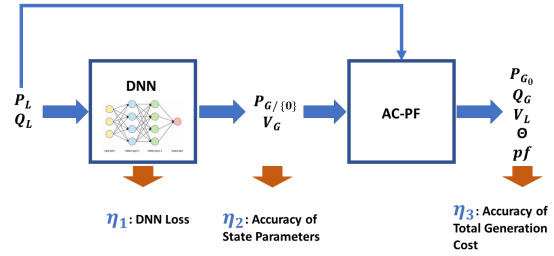
Fig. 1: The online operation framework of DNN based OPF predictor
