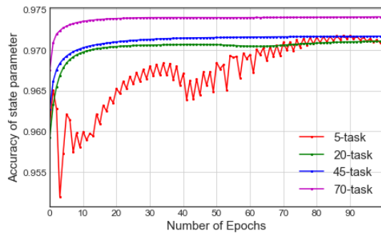
Fig. 7: Test case under IEEE-118 bus system, with \{5, 20, 45, 70\} tasks in offline training phase and training based on 50 samples from new task. The assessment is based on \eta_2 : accuracy of state parameter. Each model is updated according to 'SGD' optimization. The learning rate is 0.1 and weight decay is 0.001.
