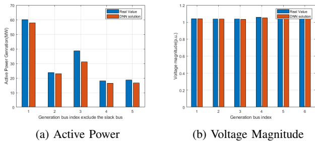
Fig. 3: Comparison of real and predicted state parameters in IEEE-30 bus system.
