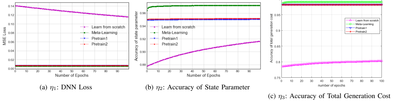
Fig. 8: Visualization of online training progress based on 50 training samples from the new task. Comparison of MTL with other benchmarks using the different metrics for IEEE-14 bus system. Learning rate = 0.001, Weight decay = 0.001.
