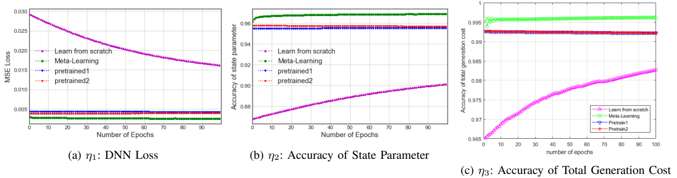
Fig. 9: Visualization of online training progress based on 50 training samples from the new task. Comparison of MTL with other benchmarks using the different metrics for IEEE-30 bus system. Learning rate = 0.01, Weight decay = 0.001.
