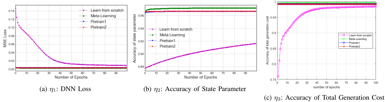
Fig. 4: Visualization of online training progress based on 50 training samples from the new task. Comparison of MTL with other benchmarks using the different metrics for IEEE-118 bus system.
