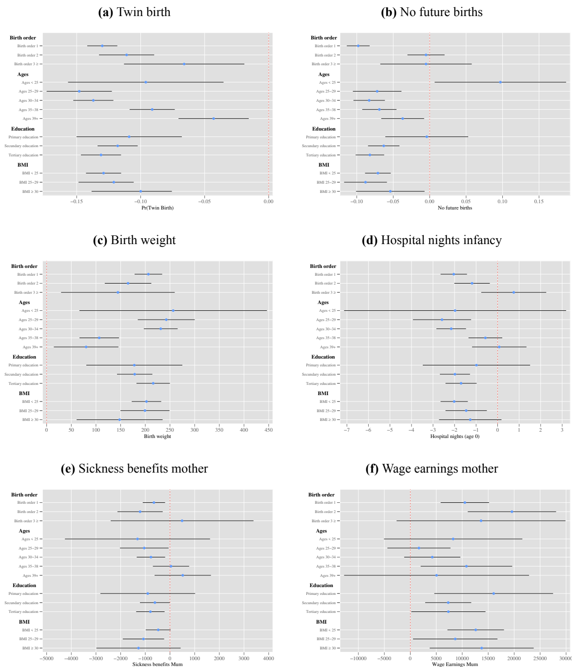
Figure 10: Reform Heterogeneity
