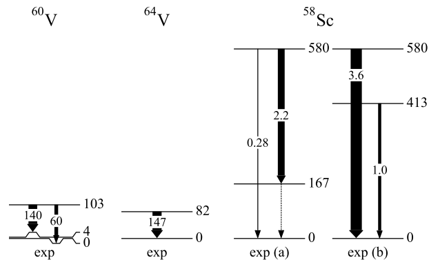
FIG. 4. Level schemes of the three nuclei discussed in the present work. States are labeled with their excitation energies in keV. The arrows indicate the observed transitions with their respective reduced transition probabilities in units of e^2\text{fm}^4 for the E2 decays in ^{60,64}\text{V} and \mu^2\text{fm}^2 for the case of ^{58}\text{Sc} with M2 transitions inferred from the lifetime measurements.
