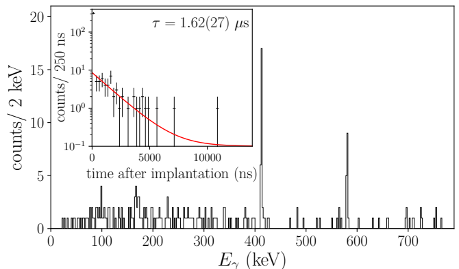
FIG. 3. Decay of the isomeric state in ^{58}\text{Sc} . Two transitions are clearly observed in the spectrum and indication for another one at 167 keV matches their difference. The inset shows the decay time distribution gated on both the 413 and 580 keV transitions.
