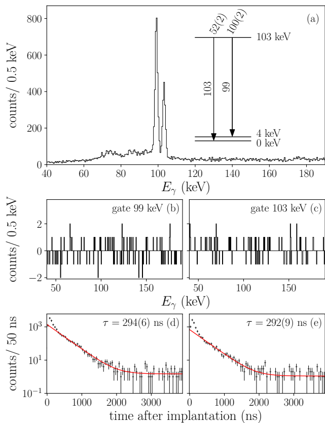
FIG. 1. Decay of the isomeric state in ^{60}\text{V} . Panel (a) shows the \gamma -ray energy spectrum in delayed coincidence with the implantation of ^{60}\text{V} . Panel (b) and (c) show the coincidence spectrum gated on each of the transitions, and panels (d) and (e) show the decay time curves together with a fit. The spectra in panels (a-c) exclude the prompt \gamma flash which dominates the spectra for t < 300 ns. The fits in panels (d) and (e) also exclude early times.
