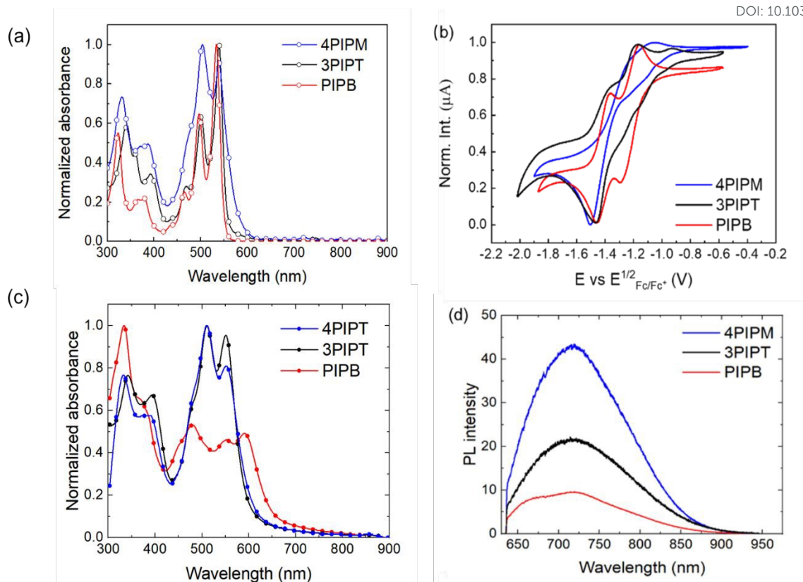
Figure 3. (a) Normalized optical absorption of 5 \times 10^{-6} M solutions in chloroform, (b) cyclic voltammograms measured in dichloromethane, (c) normalized solid state UV-Vis absorption spectra and (d) photoluminescence spectra of PIPB (red), 3PIPT (black) and 4PIPM (blue) films.
