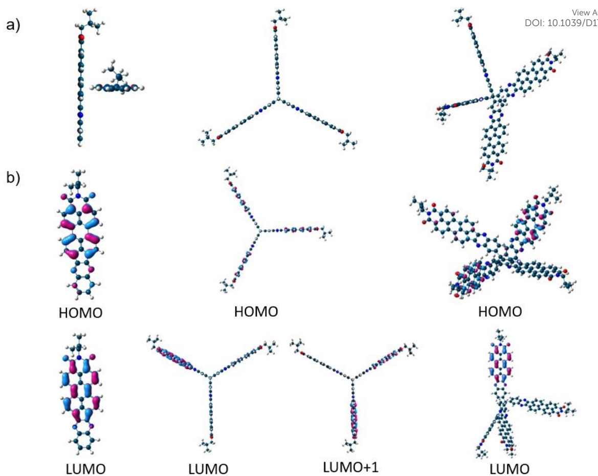
Figure 2. (a) G16 DFT/B3LYP/6-31* optimized molecular structures for the semiconductors under study and (b) molecular orbital topologies of PIPB (left), 3PIPT (middle) and 4PIPM (right).
