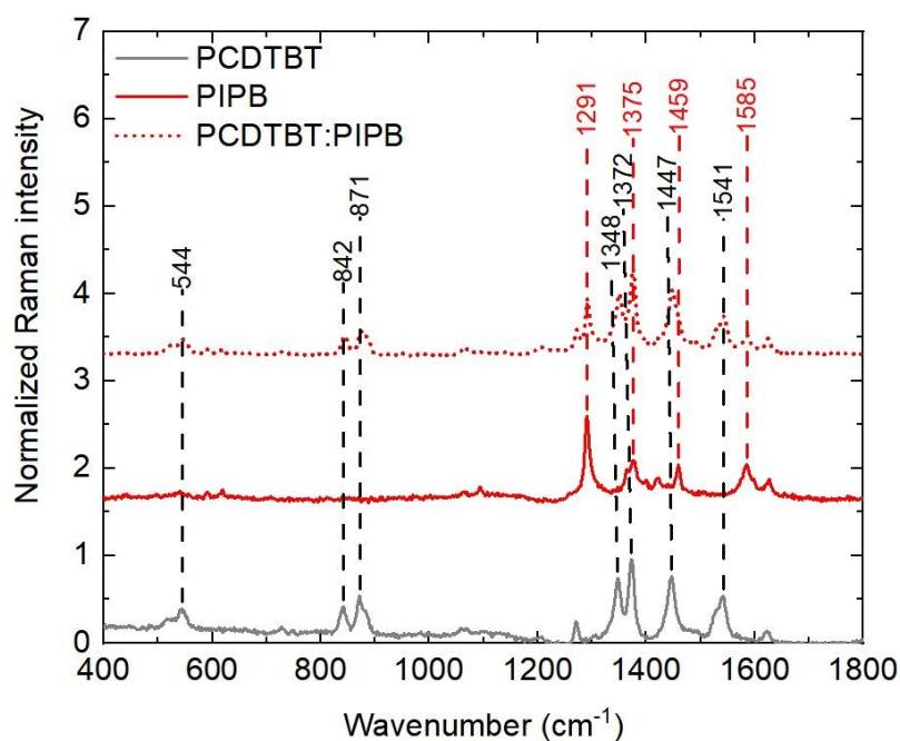
Figure 7. Raman spectra of PCDTBT (grey), PIPB (red) and PCDTBT:PIPB (dotted red).
