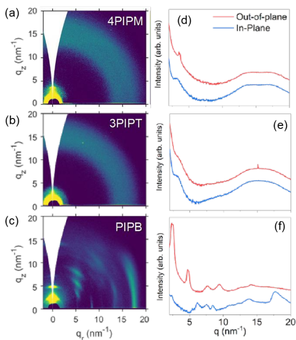
Figure 4. 2D GIWAXS patterns and the out-of-plane (OOP, red line) and in-plane (IP, blue line) cuts of the corresponding 2D-GIWAXS patterns of the three acceptors 4PIPM (a and d), 3PIPT (b and e) and PIPB (c and f).
