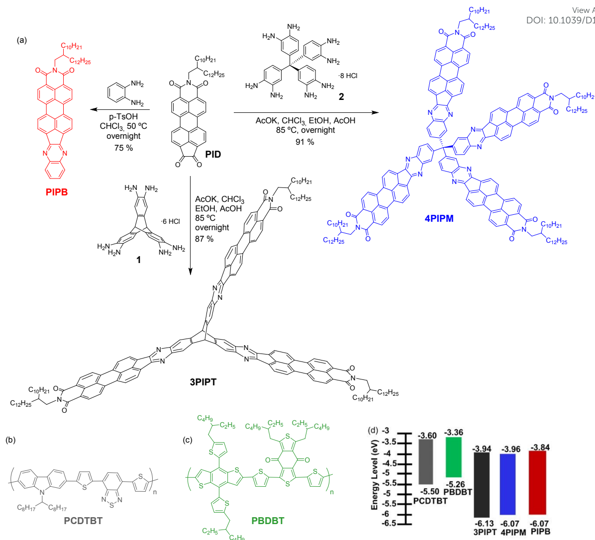
Figure 1. (a) Synthesis of PIPB , 3PIPT and 4PIPM ; the molecular structure of (b) PCDTBT , (c) PBDBT and (d) the energy levels of all the molecules deduced from cyclic voltammetry and UV-Visible.
