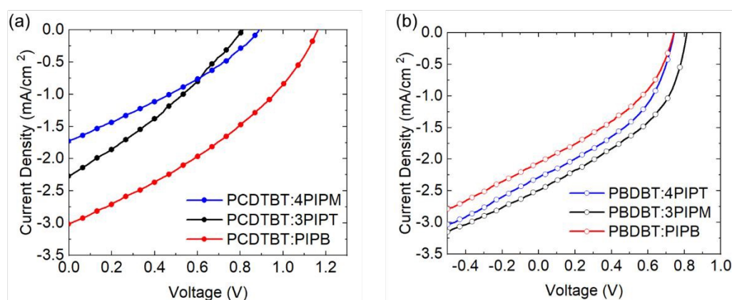
Figure 8. (a) The J–V curves of the champion PV devices with PCDTBT donor polymer and (b) the J–V curves of the champion PV devices with PBDBT donor polymer.
