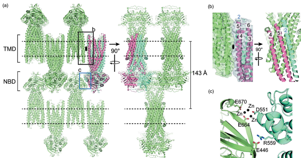
Figure 2 Type I crystal packing of the CmABCBC1 OTA OF crystal structure. (a) Crystal packing of CmABCBC1 OTA molecules shows alternating layers of antiparallel homodimers within the crystal. (b) An interface formed by the TM2, TM4 and TM5 helices of two CmABCBC1 OTA dimers. (c) Major interactions at the NBD interface.
