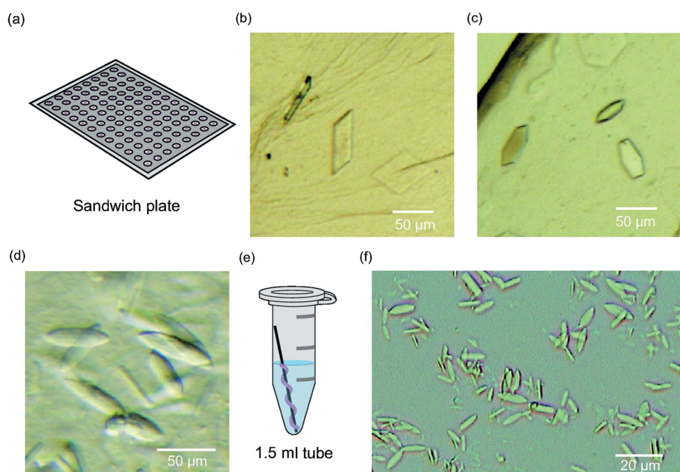
Figure 1 LCP crystals of CmABCB1. (a) A diagram of the 96-well glass sandwich plate used for LCP crystallization. (b) Rectangular plate crystals, (c) hexagonal plate crystals and (d) leaf-shaped crystals of CmABCB1 OTA formed on the glass sandwich plate. (e) A diagram depicting batch LCP crystallization of CmABCB1 in a 1.5 ml tube. (f) Microcrystals of CmABCB1 OTA formed using the batch method.
