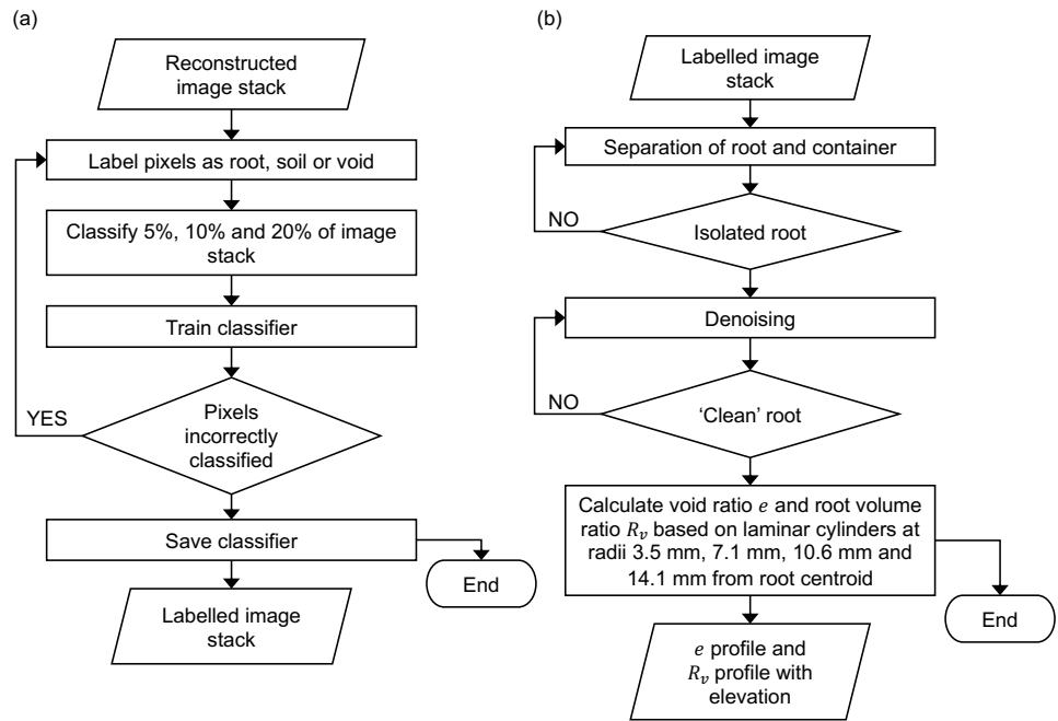
Figure 3. Flow charts representing the algorithmic steps of: (a) automatic classification process using deep learning (b) the MATLAB parameter quantification process.
