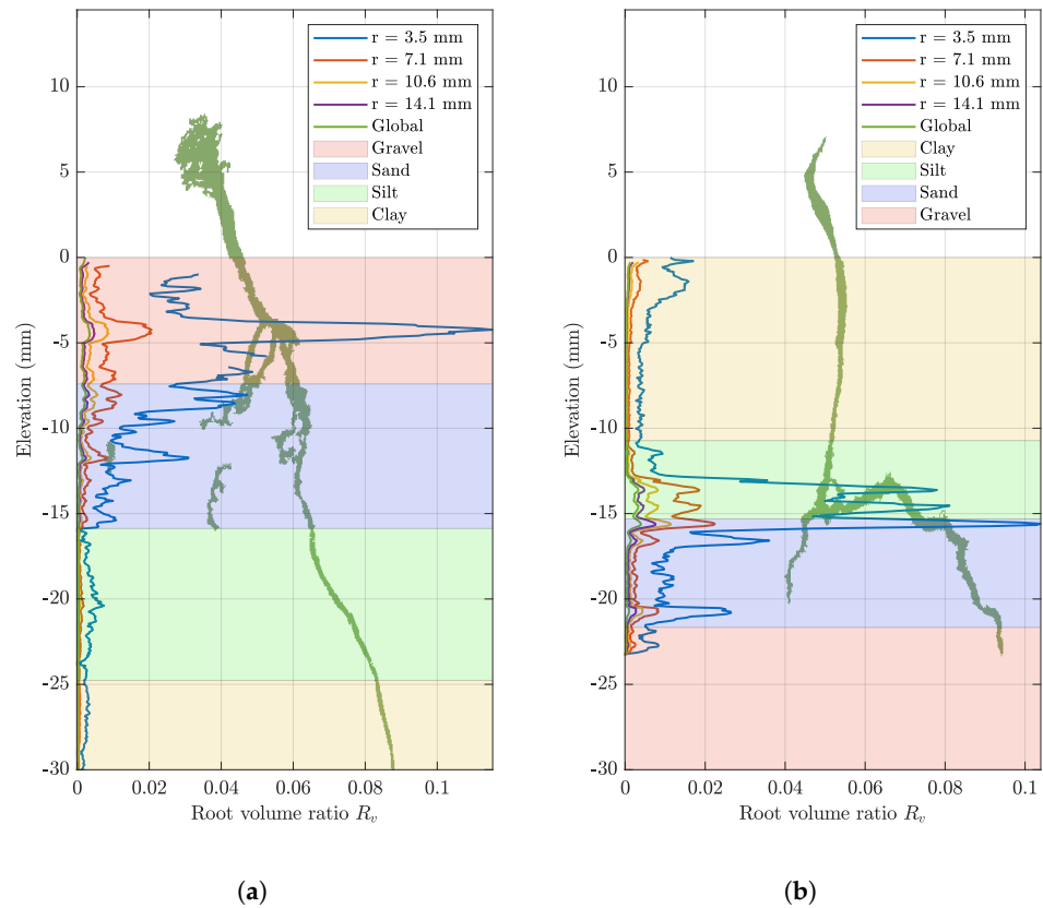
Figure 7. Root volume ratio profiles with elevation of (a) sample A, day 15 and (b) sample B, day 15, using the 10% classifier (the layer thickness corresponds to averaged elevation for each stratum).
