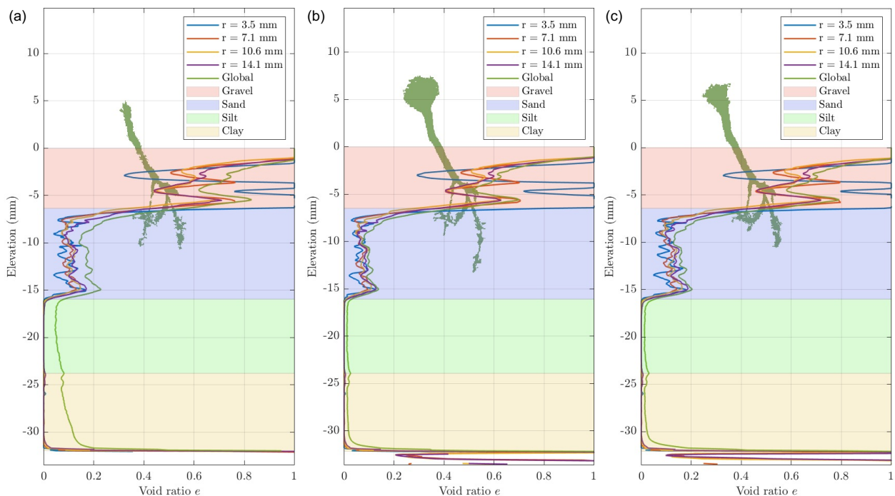
Figure 8. Void ratio profiles with elevation for sample A, day 11 using the classifier trained based on (a) 5%, (b) 10%, and (c) 20% of the image stacks (the layer thickness corresponds to averaged elevation for each stratum).
