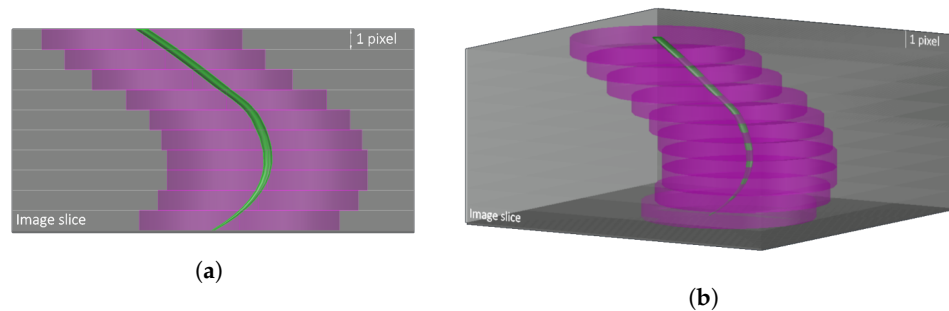
Figure 4. Schematic of laminar cylinder around root used as region of interest (ROI) to calculate parameters of geotechnical interest for varying elevation: (a) side view (b) perspective view.
