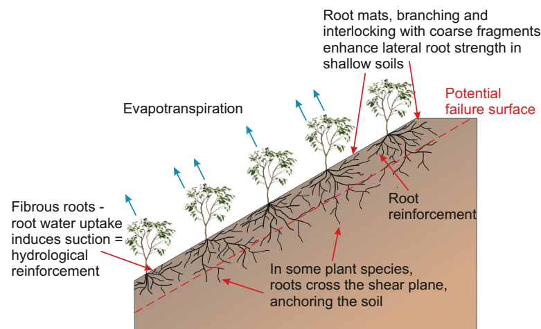
Figure 1. Root reinforcement in slope stability (inspired from [5]).
