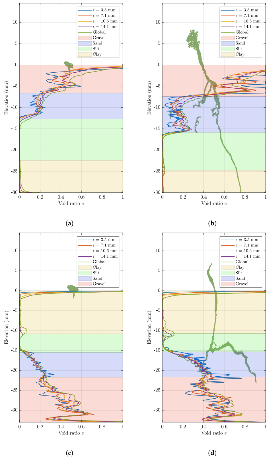
Figure 6. Void ratio profiles with elevation of (a) Sample A, day 1, (b) sample A, day 15, (c) sample B, day 1, and (d) sample B, day 15, using the 10% classifier (the layer thickness corresponds to averaged elevation for each stratum).
