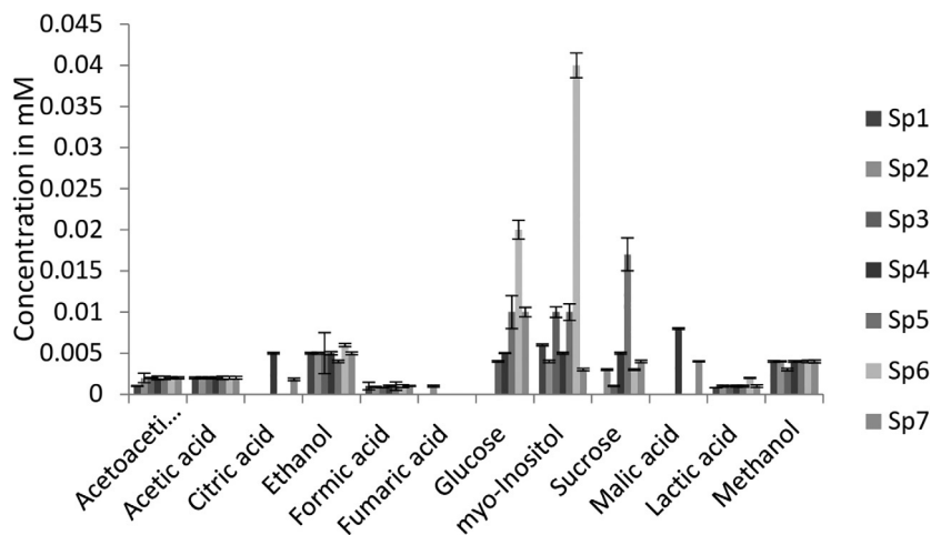
Fig. 4 ^1\text{H} NMR average quantification of compounds of Drosera biofluids. Sp1: Drosera adalae , Sp2: Drosera regia , Sp3: Drosera capensis Alba, Sp4: Drosera capensis Giant, Sp5: Drosera capensis Rubra, Sp6: Drosera binata , Sp7: Drosera slackii ( n=3 with standard deviation).
