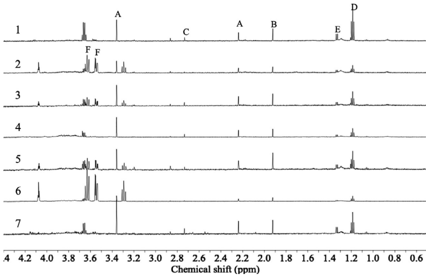
Fig. 2 ^1\text{H} NMR spectra of seven Drosera species (600 MHz, \text{KH}_2\text{PO}_4 buffer containing 0.01% trimethylsilylpropanoic acid (TMSP, w/w) in the range of \delta 0.3–4.5. 1. Drosera adaelae , 2. Drosera regia , 3. Drosera capensis Alba, 4. Drosera capensis Giant, 5. Drosera capensis Alba, 6. Drosera capensis Rubra, 7. Drosera binata , 7. Drosera slackii . A: acetoacetic acid, B: acetic acid, C: citric acid, D: ethanol, E: lactic acid, F: myo -inositol.
