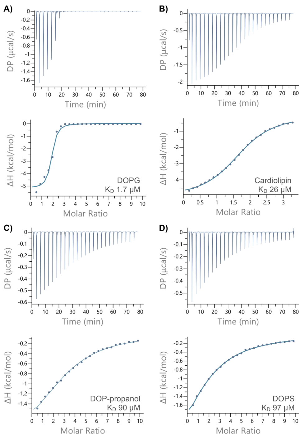
Figure 2. Representative binding isotherms for the titrations of 10 mM DOPC LUVs containing 25 mol % of: (A) DOPG (titrated into 50 \mu\text{M} daptomycin); (B) cardiolipin (titrated into 150 \mu\text{M} daptomycin); (C) DOP-propanol and (D) DOPS (both titrated into 50 \mu\text{M} daptomycin). Buffer used for all binding experiments consisted of 20 mM HEPES, 5 mM \text{CaCl}_2 , 150 mM NaCl, pH 7.4.
