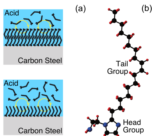
Figure 1 (a) Cartoons of organic corrosion inhibitor species forming a monolayer (bottom) or bilayer (top) on a metallic substrate (carbon steel) in acidic solution. The yellow circles with arrows indicate that the adsorbed layers are dynamic, i.e., they dissipate in the absence of corrosion inhibitor in the bulk solution. (b) Ball and stick model of OMID, where the black, blue, and red spheres represent carbon, nitrogen, and hydrogen atoms, respectively. The Head Group, which is expected to be involved in substrate bonding, comprises a heterocyclic ring (C 3 N 2 H 4 ) and a pendant side group (C 2 H 4 NH 2 ). The Tail Group is an unbranched aliphatic chain (C 17 H 33 ).
