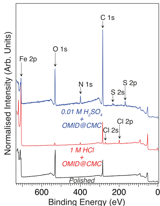
Figure 3 Overview XPS spectra ( h\nu = 1486.6 eV, \theta_E = 0^\circ ) acquired from carbon steel subsequent to immersion for 4 h in either 1M HCl/OMID (red line) or 0.01M H 2 SO 4 /OMID (blue line). The bottommost spectrum (black line) was acquired from a polished carbon steel substrate.
