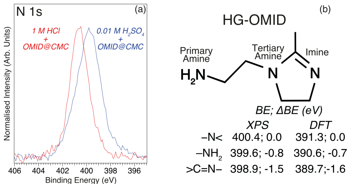
Figure 4 (a) N 1s core level XPS spectra ( h\nu = 1486.6 eV, \theta_E = 0^\circ ) acquired from carbon steel following immersion for 4 h in either 1M HCl/OMID (red line) or 0.01M H 2 SO 4 /OMID (blue line). (b) Skeletal model of OMID head group (HG-OMID), and BEs, plus \Delta BEs relative to -N<, for each nitrogen atom, derived from either XPS or DFT calculations.
