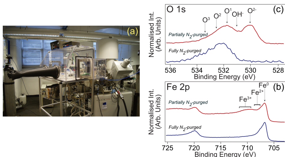
Figure 2 (a) Photograph of N_2 -filled glove box attached to load lock of XPS spectrometer to allow transfer of samples without post-immersion air exposure. This setup was employed for all XPS data presented in this study. (b) Fe 2p XPS spectra ( h\nu = 1486.6 eV, \theta_E = 0^\circ ) acquired from carbon steel samples that had been immersed in 1 M HCl inhibited with MBI [12,13]. The blue (red) spectrum is from a sample transferred through a fully (partially) N_2 -purged glove box [12,13]. (c) O 1s XPS spectra acquired under analogous conditions; O 1 , O 2 and O 3 arise from adsorbed OH (O 1 ) and an adventitious carbon layer (O 1 – O 3 ).
