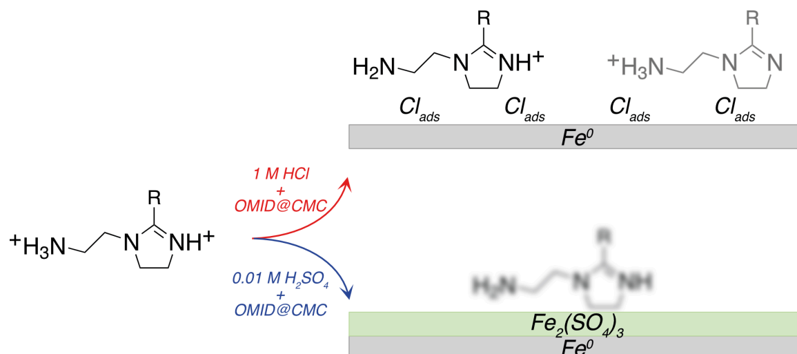
Figure 8 Cartoon summarising interpretation of N 1s, Fe 2p, O 1s, Cl 2p, and S 2p XPS spectra acquired from carbon steel following immersion for 4 h in either 1M HCl/OMID or 0.01M H 2 SO 4 /OMID. For 1M HCl/OMID, two OMIDH + species are concluded to be adsorbed onto a oxide/salt-free surface, decorated with chlorine atoms. For 0.01M H 2 SO 4 /OMID, the exact nature of the adsorbed OMID remains ill-defined, but it is adsorbed onto an ultra-thin oxide/salt film, composed primarily of a ferric sulfate (Fe 2 (SO 4 ) 3 )-like phase. R = C 17 H 33 .
