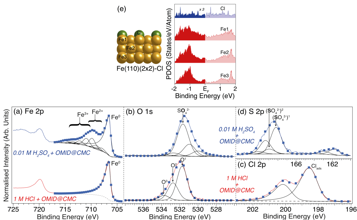
Figure 7 (a) Fe 2p, (b) O 1s, (c) Cl 2p and (d) S 2p core level XPS spectra acquired from carbon steel following immersion for 4 h in either 1M HCl/OMID (lower row) or 0.01M H 2 SO 4 /OMID (upper row). Spectra have been normalised such that minima are 0, and maxima are 1. Blue markers show best fits to the experimental spectra (solid red/blue lines), using GL (black lines), LF (black lines), and Shirley-type (broken grey lines) functions. Peak assignments are also indicated. For the Cl 2p and S 2p spin-orbit split doublets ( 2p_{1/2} and 2p_{3/2} ), the BE differences and intensity ratios are consistent with expected values [11]. (e) On the left, side view of the structure of ordered (2x2) overlayer of Cl atoms on Fe(110), that was optimised in DFT calculations to produce PDOS for Cl, Fe1, Fe2, and Fe3. The corresponding PDOS are plotted on the right; both Fe and Cl display finite PDOS around E_F .
