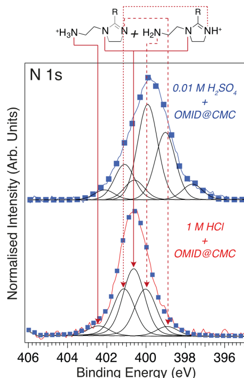
Figure 5 N 1s core level XPS spectra ( h\nu = 1486.6 eV, \theta_E = 0^\circ ) acquired from carbon steel following immersion for 4 h in either 1M HCl/OMID (lower spectrum) or 0.01M H 2 SO 4 /OMID (upper spectrum). Blue markers show best fits to the experimental spectra (red/blue lines), using GL(30) (black lines) and Shirley-type (broken grey lines) functions. Peak assignments, consistent with OMID being adsorbed on carbon steel in 1M HCl/OMID in the two OMIDH + forms shown at the top of this figure, are also indicated. R = C_{17}H_{33} .
