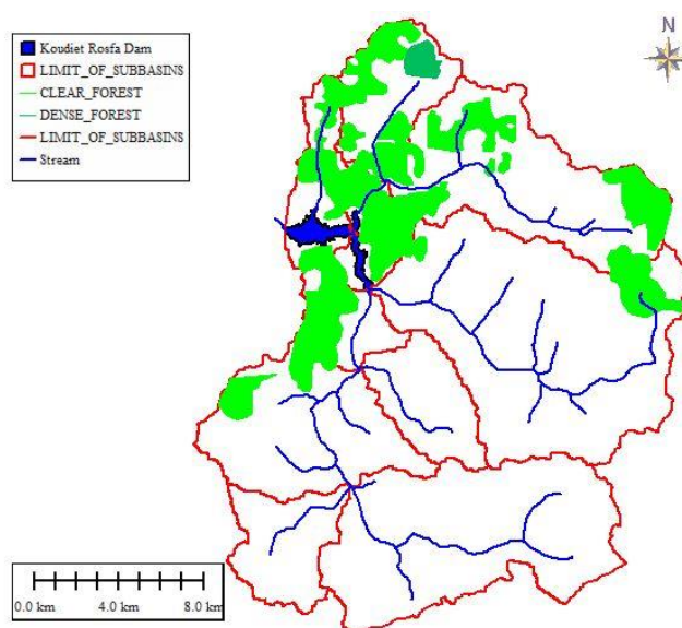
Figure 2. Land use of Koudiet Rosfa watershed
