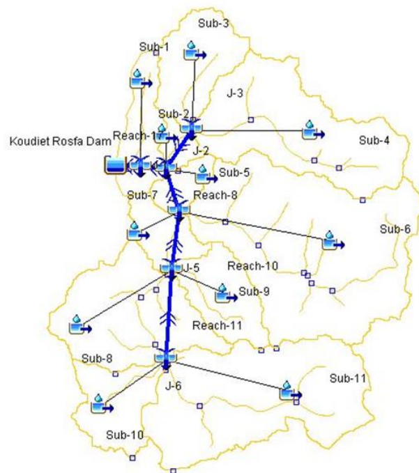
Figure 4. HEC-HMS model for Koudiet Rosfa watershed
