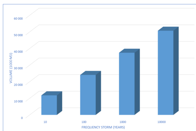
Figure 8. Resulting volume of hypothetical frequency storms
