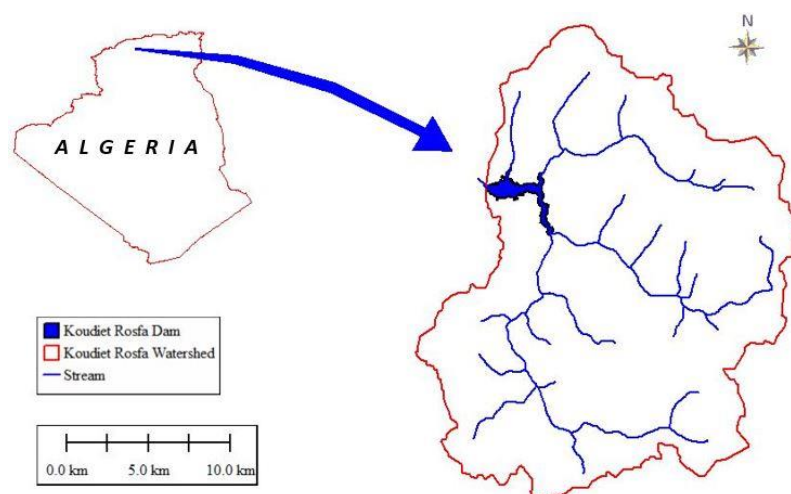
Figure 1. Koudiet Rosfa watershed
