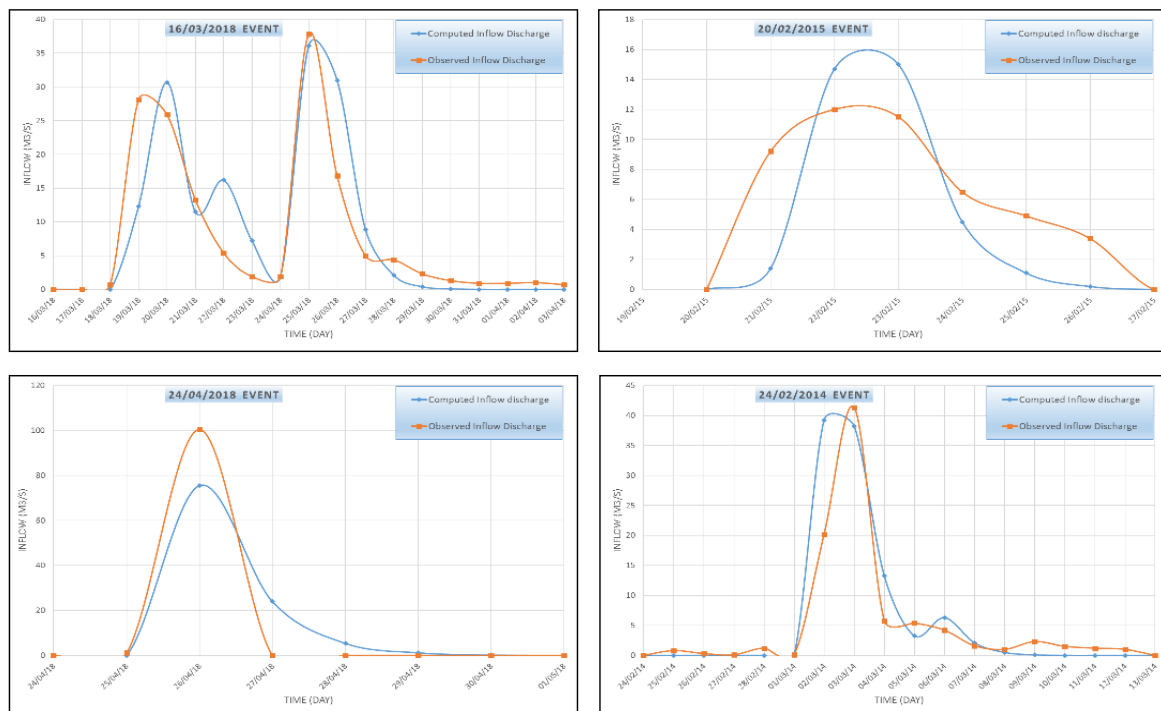
Figure 6. Resulting hydrographs
