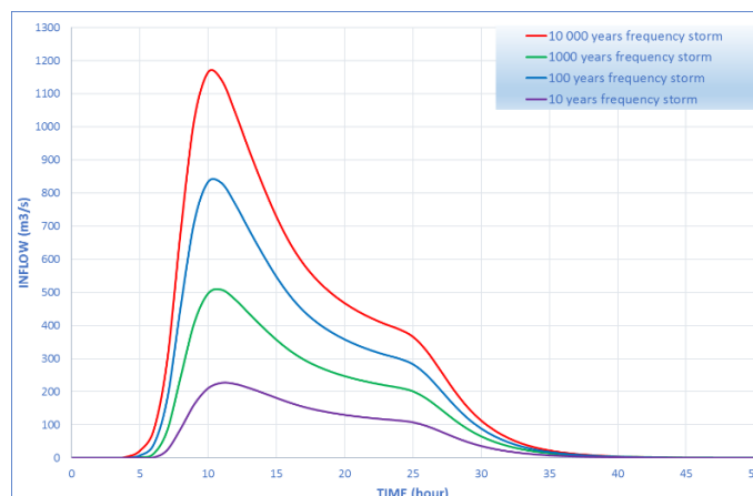
Figure 7. Inflow discharges of hypothetical frequency storms
