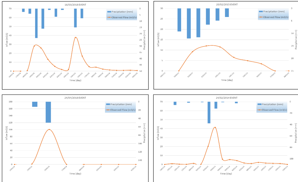
Figure 5. Hydrological events for model calibration
