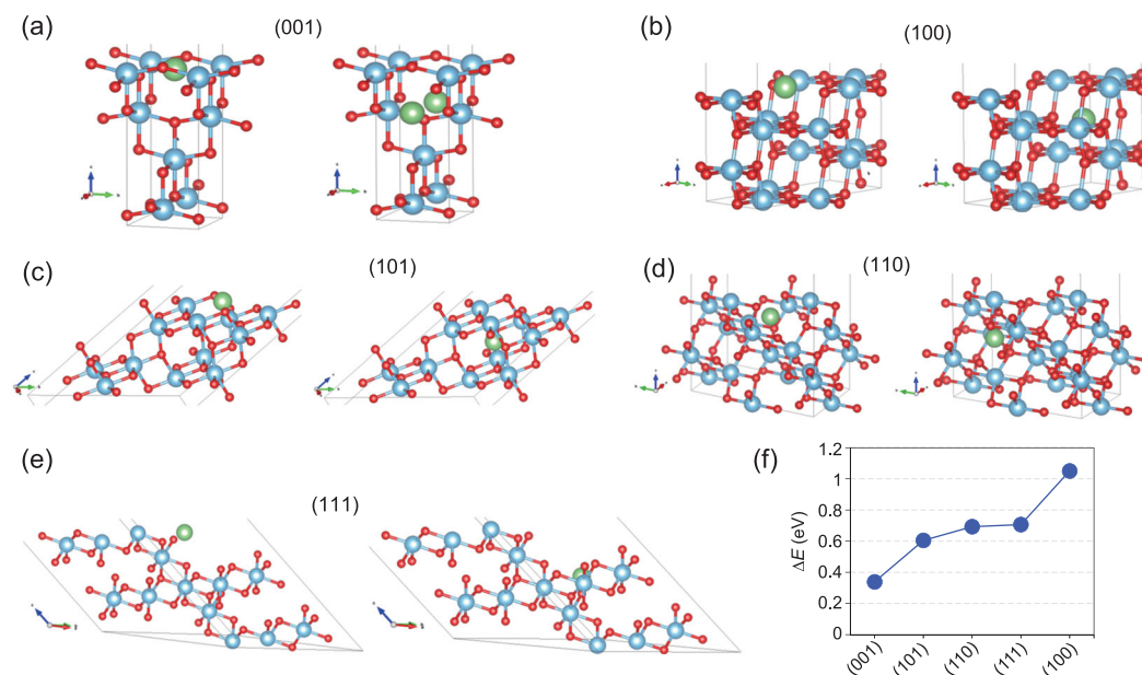
Figure 1. Crystal models for Li ions migrating from various crystal surfaces to the internal octahedral voids. Left (initial state) and right (final state): (a) (001), (b) (100), (c) (101), (d) (110) and (e) (111) crystal plane surfaces. (f) The calculated energy barriers for the corresponding crystal planes. Li ions are in green, Titanium atoms are in blue and oxygen atoms are in red.
