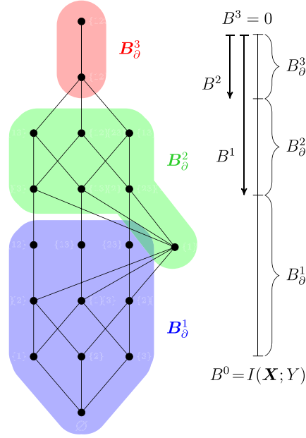
Figure 3. Schematic representation of the backbone lattice. (left) Correspondence between backbone atoms and S_{\theta}^{\alpha} for the n = 3 lattice. (right) Representation of the backbone lattice as a totally ordered set.
