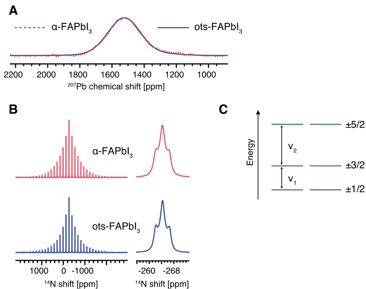
Fig. S13. (A) Solid-state 207 Pb NMR shows that the main component of EDTA-doped FAPbI 3 is \alpha -FAPbI 3 . (B) 14 N MAS NMR is highly sensitive to the symmetry of the A-site cation cage of the 3D perovskite phase. Here, it is not sensitive enough to detect any differences in symmetry between \alpha -FAPbI 3 and ots-FAPbI 3 . Data recorded at 4 kHz MAS (full sideband pattern, left) and 12 kHz (central peak, right). (C) The energy level diagram for Nuclear Quadrupole Resonance (NQR) of 127 I in a zero applied magnetic field. In the case of \alpha -FAPbI 3 , v_1 = 86.606 MHz, v_2 = 173.217 MHz. \pm 5/2 , \pm 3/2 and \pm 1/2 indicate the possible spin states.
