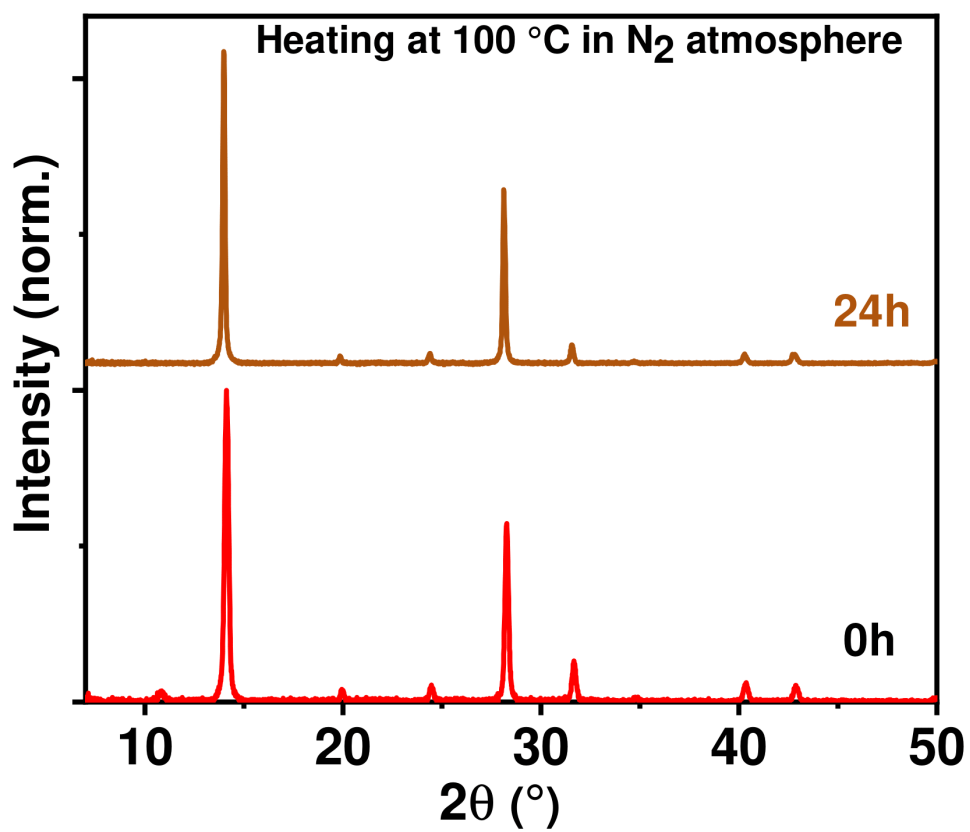
Fig. S17 XRD patterns for thin films of an \text{ots-FAPbI}_3 thin film before and after heating at 100 °C in \text{N}_2 atmosphere for 24 hours.
