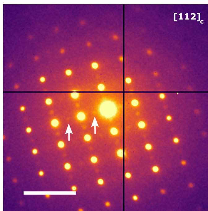
Fig. S12. Superstructure reflections indicating octahedral tilting in ots-FAPbI 3 (subset shown with white arrows) not consistent with the P4/mbm space group. Scalebar = 0.7Å -1
