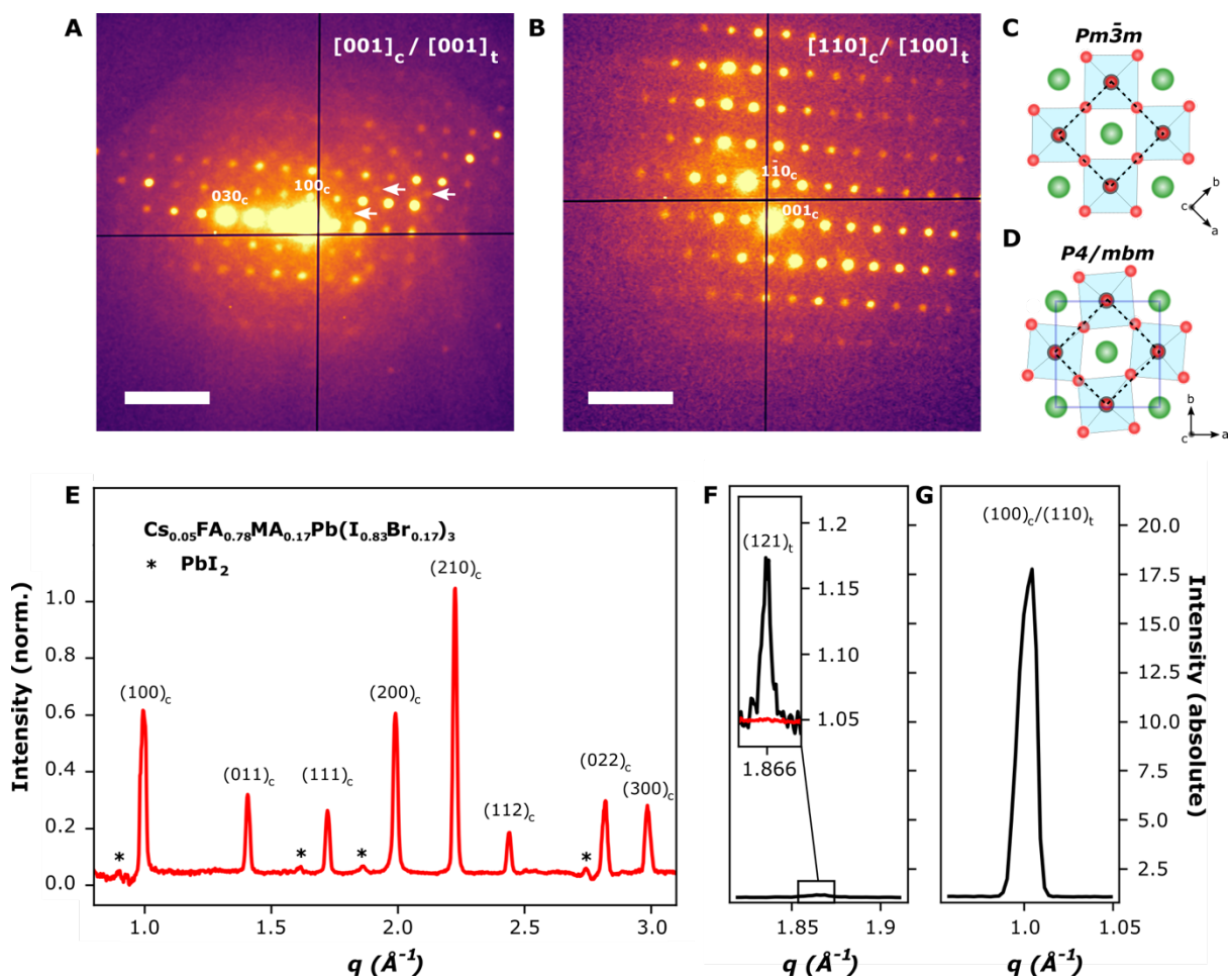
Fig. 1. Structural identification of tetragonal Cs_{0.05}FA_{0.78}MA_{0.17}Pb(I_{0.83}Br_{0.17})_3 thin films. (A) The ED pattern of a Cs_{0.05}FA_{0.78}MA_{0.17}Pb(I_{0.83}Br_{0.17})_3 sample oriented near the [001] zone
