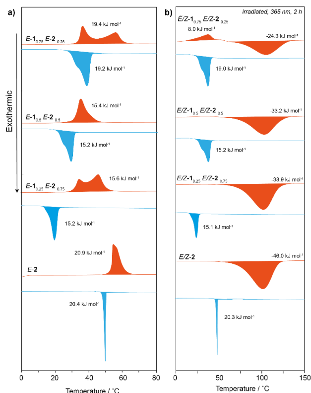
Figure 2. DSC first heating branches (red) and first cooling branches (blue) of a) E - 1 x E - 2 (1- x ) , and b) irradiated E/Z - 1 x E/Z - 2 (1- x ) composites. Thermograms were obtained at a heating rate of 2.5 °C min -1 .
