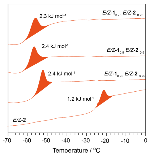
Figure 3. DSC first heating branches (red) of irradiated E/Z-1 x E/Z-2 (1-x) composites. Thermograms were obtained at a heating rate of 2.5 °C min -1 between -70 to 0 °C.
