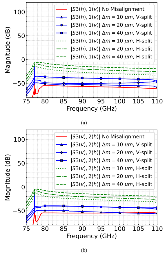
Fig. 16. Polarization isolation for (a) vertical polarization (when port 1 is excited) and (b) horizontal polarization (when port 2 is excited).
