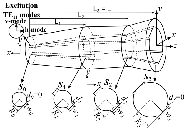
Fig. 7. Geometry of the multi-section grooved-wall CP horn.
