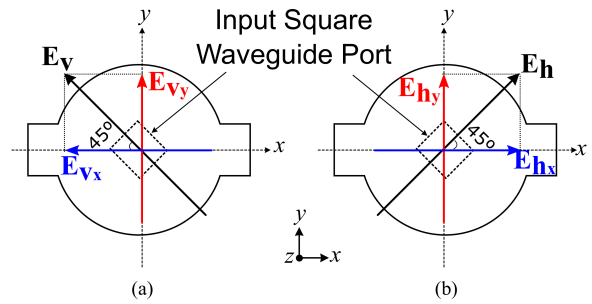
Fig. 4. The decomposition of (a) v-mode and (b) h-mode at the cross-section of grooved-wall circular waveguide.
