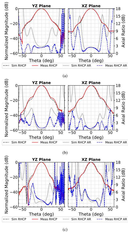
Fig. 23. Normalized measured and simulated RHCP (port 2 excited) radiation patterns of the proposed dual-CP antenna at (a) 80 GHz, (b) 95 GHz and (c) 110 GHz.
